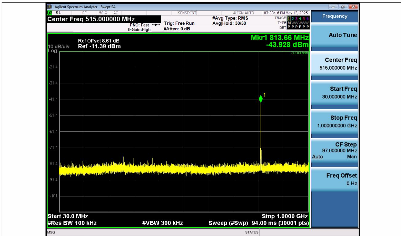
2DH5-Ant1-2441-30~1000-PASS
