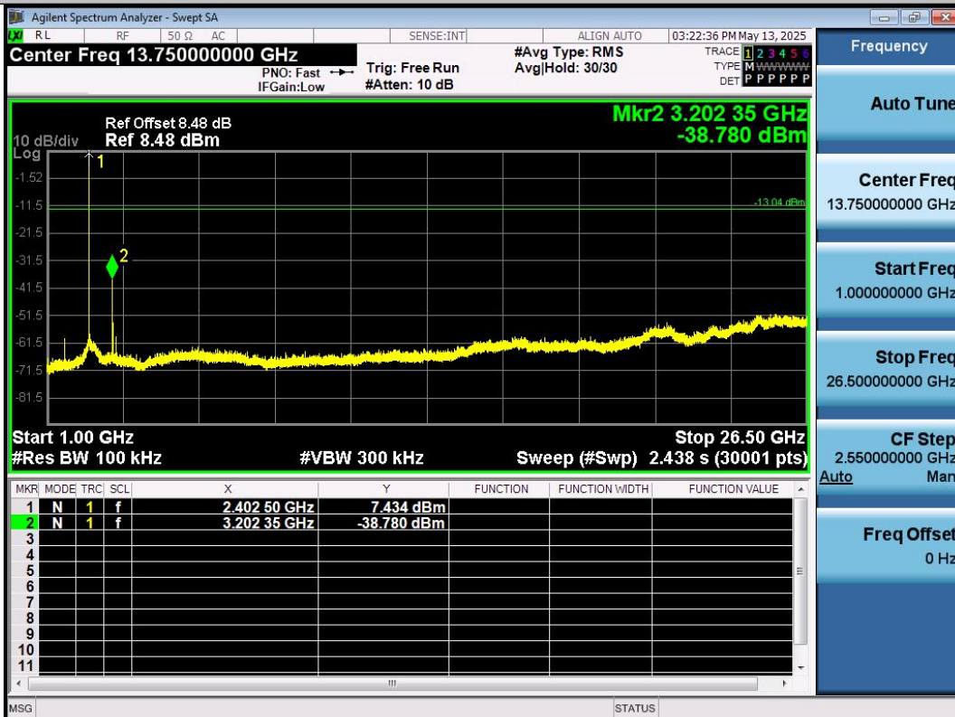
DH5-Ant1-2402-1000~26500-PASS
