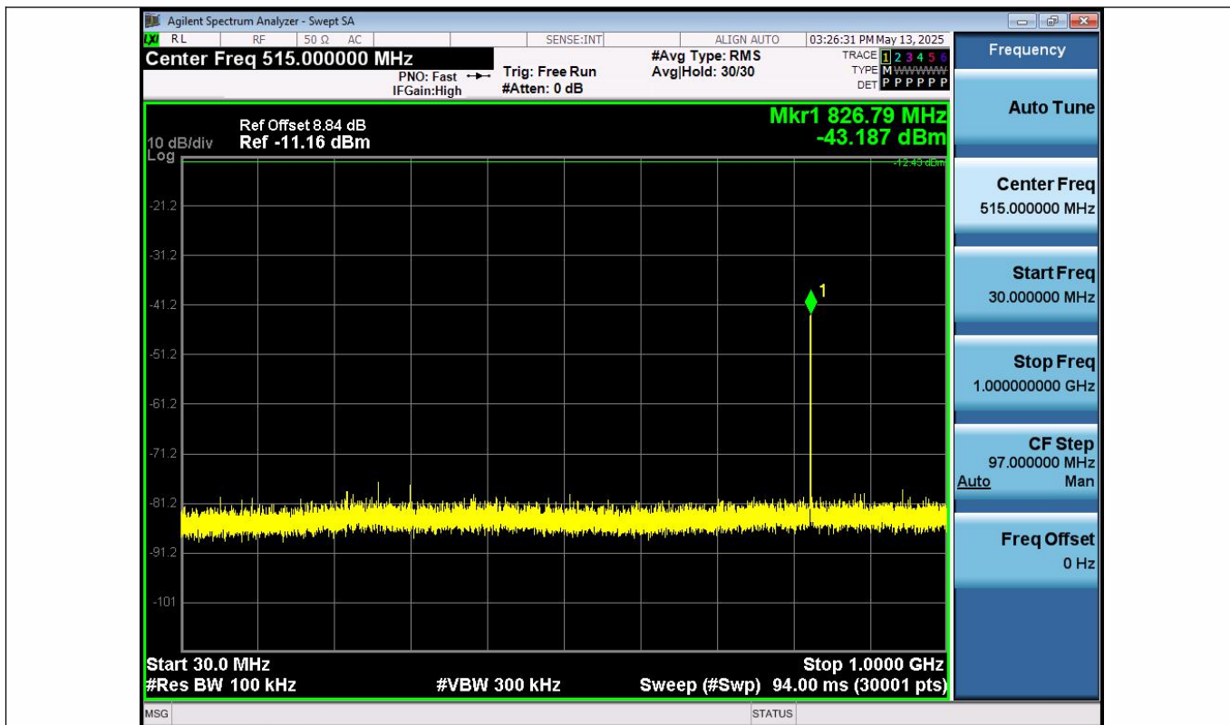
DH5-Ant1-2480-30~1000-PASS
