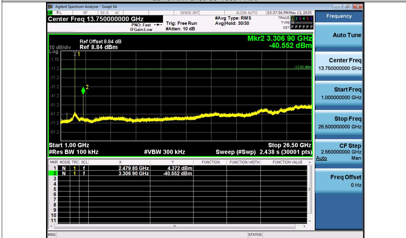
2DH5-Ant1-2480-1000~26500-PASS
