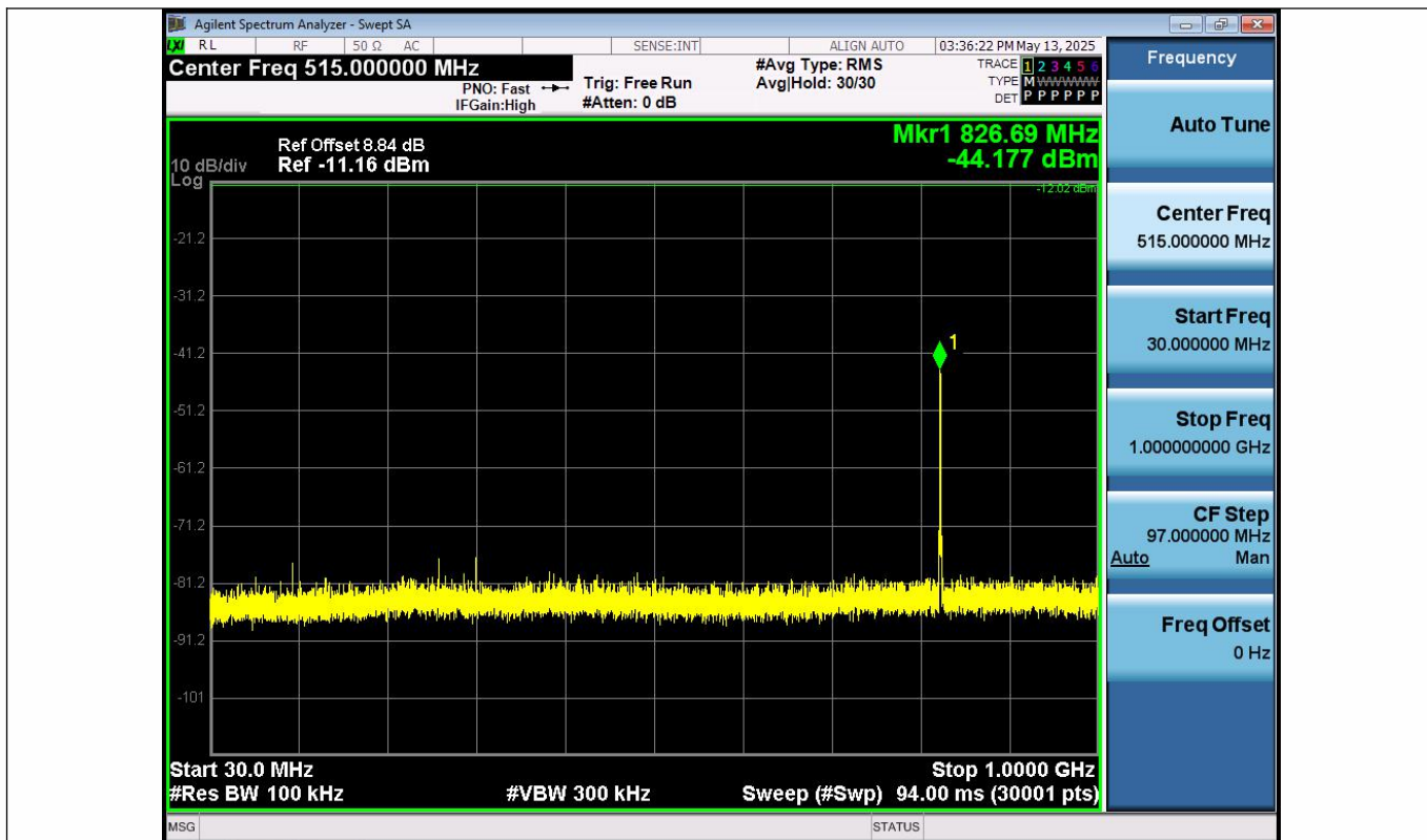
2DH5-Ant1-2480-30~1000-PASS
