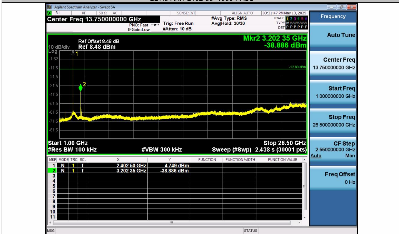
2DH5-Ant1-2402-1000~26500-PASS
