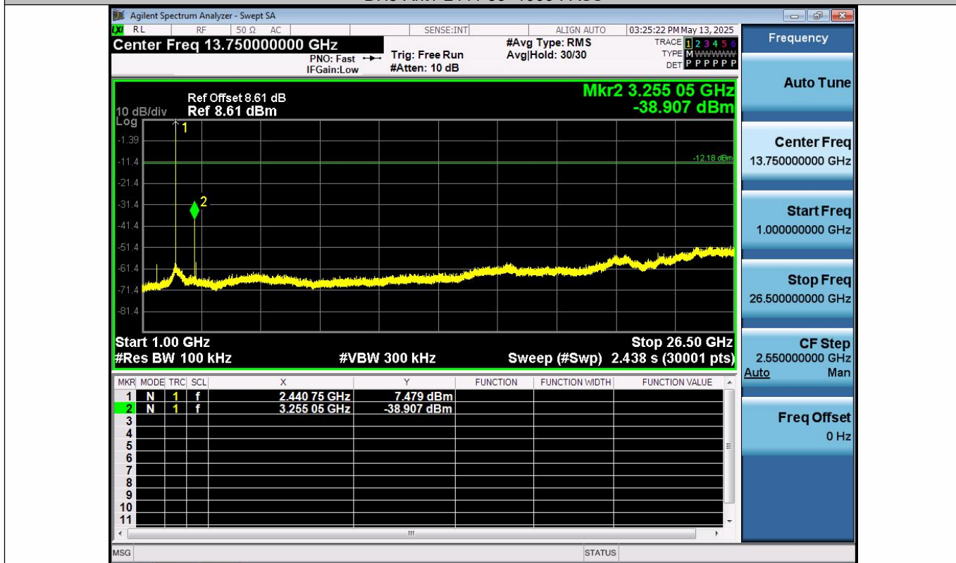
DH5-Ant1-2441-1000~26500-PASS
