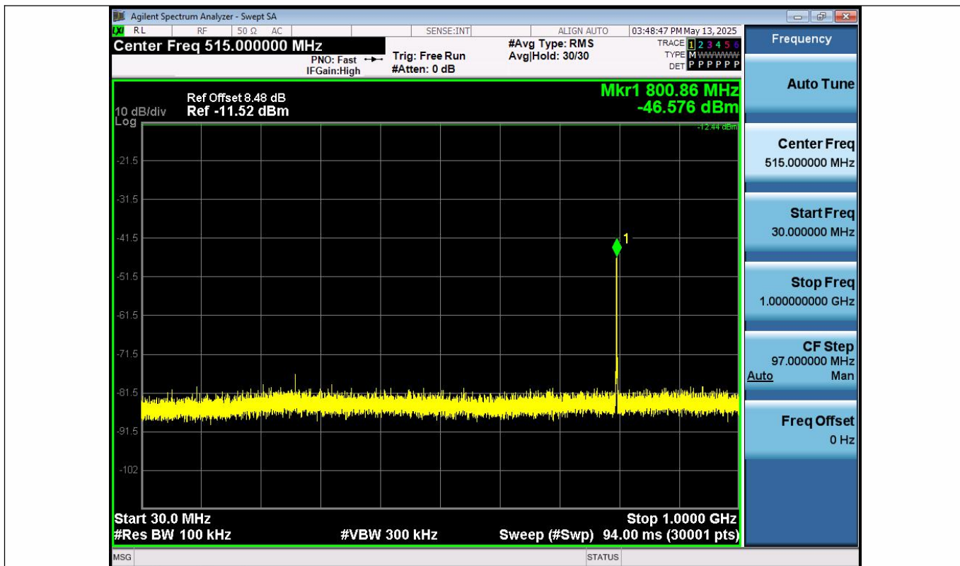
3DH5-Ant1-2402-30~1000-PASS
