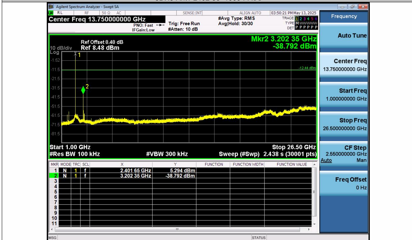
3DH5-Ant1-2402-1000~26500-PASS
