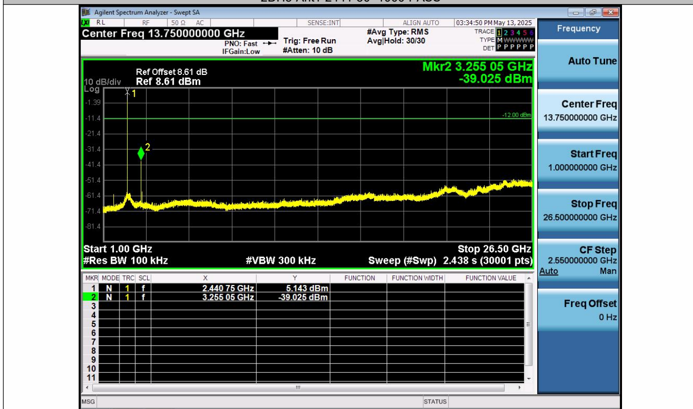
2DH5-Ant1-2441-1000~26500-PASS
