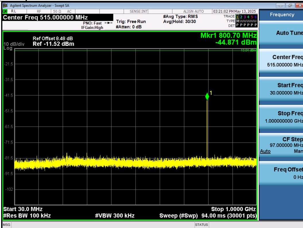
DH5-Ant1-2402-30~1000-PASS
