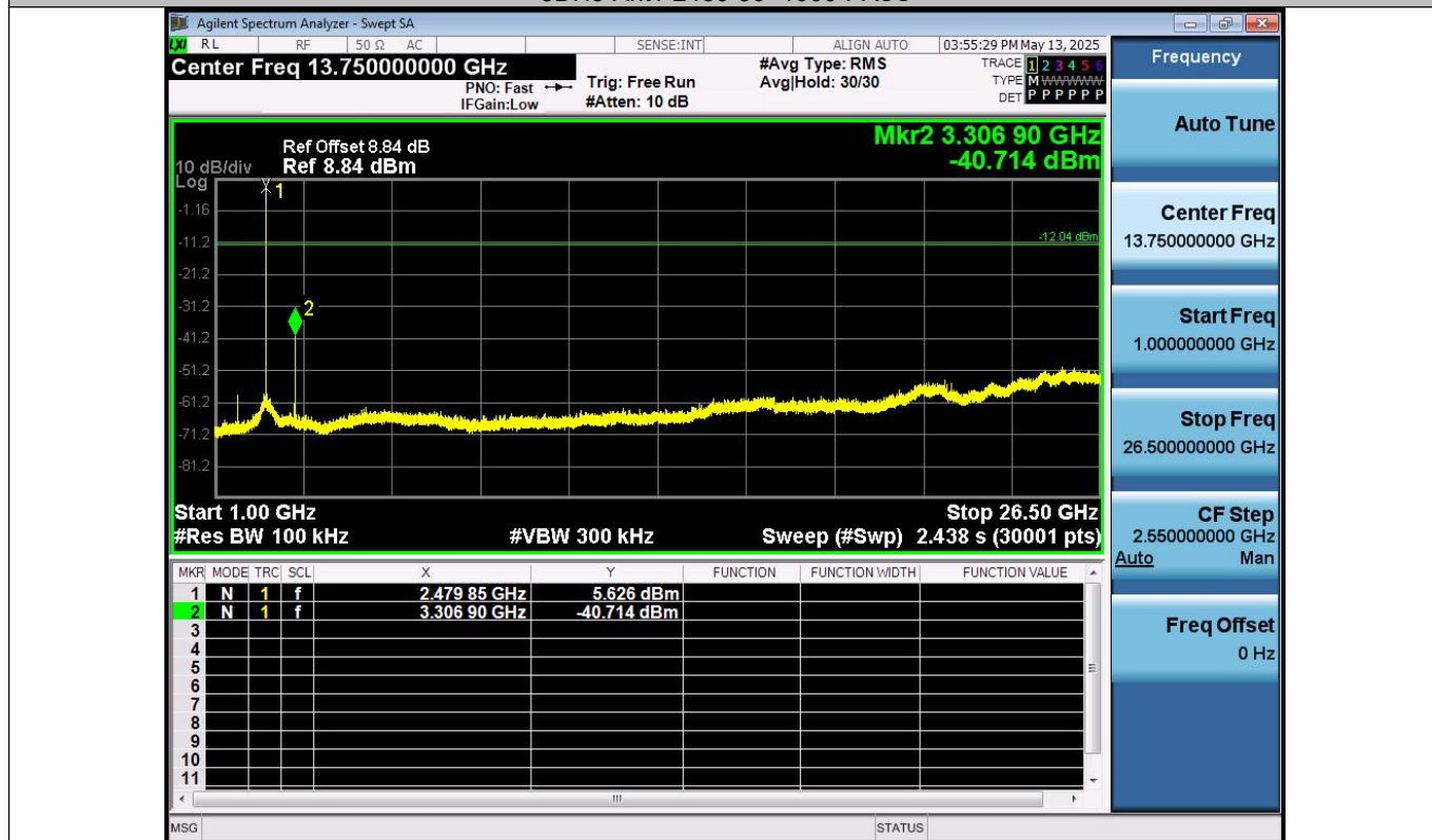
3DH5-Ant1-2480-1000~26500-PASS
