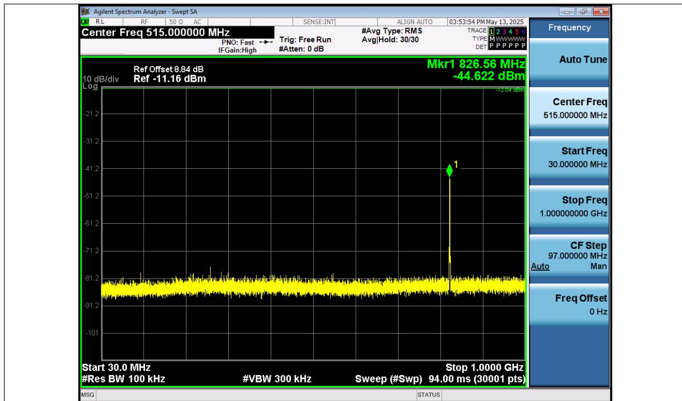
3DH5-Ant1-2480-30~1000-PASS
