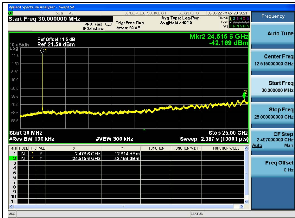
(30MHz to 25GHz, Channel 26)
