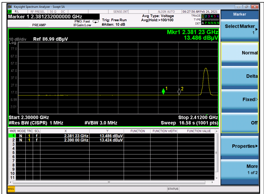
(AVERAGE, Channel 11)
