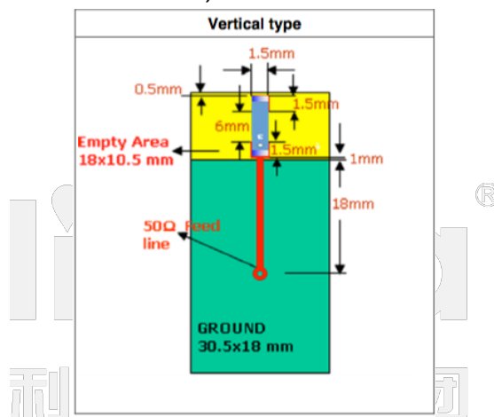
Antenna on Test Board ( FR4 Thickness 0.8mm)
