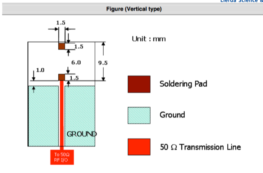
Antenna on Test Board ( FR4 Thickness 0.8mm)
