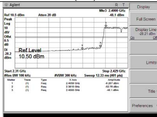
802.11 n(40M) Mode
