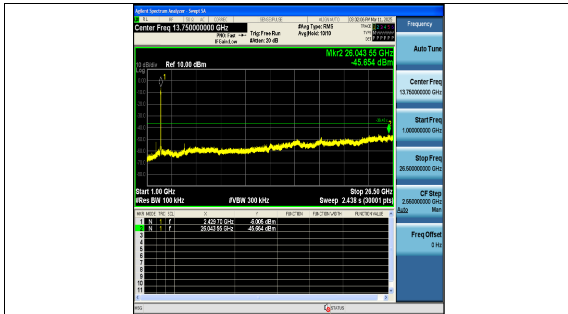
11AX40SISO-Ant1-2437-1000~26500-PASS
