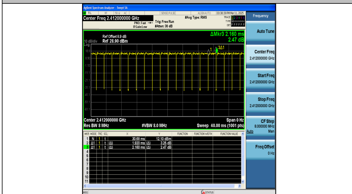
NTNV-11N20SISO-Ant1-2412
