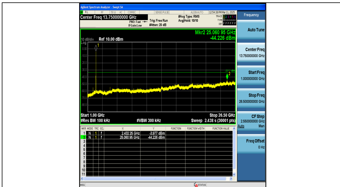
11AX20SISO-Ant1-2437-1000~26500-PASS
