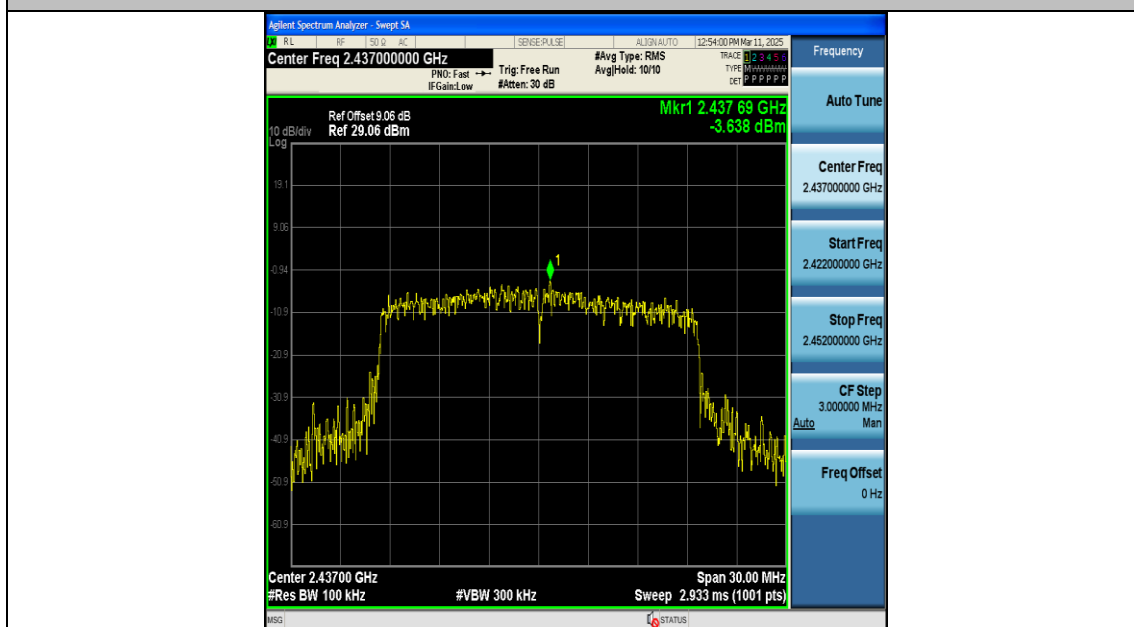
11AX20SISO-Ant1-2437-0~Reference-PASS
