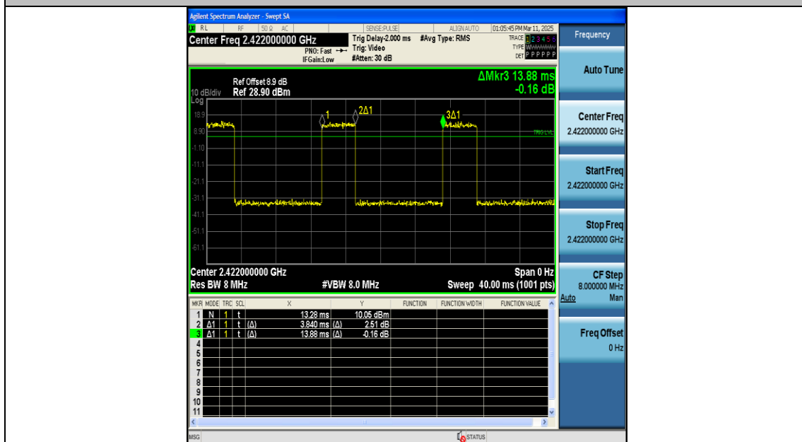
NTNV-11AX40SISO-Ant1-2422
