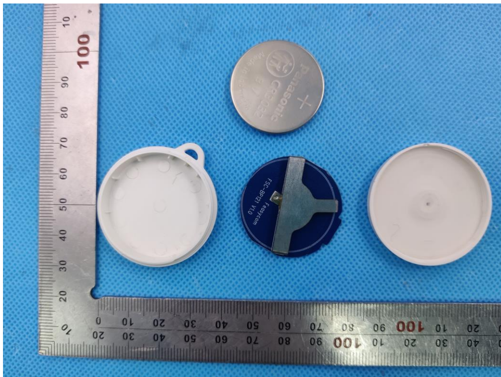
With battery 2: 3V 500mA OPEN VIEW OF EUT (FIGURE 1)
