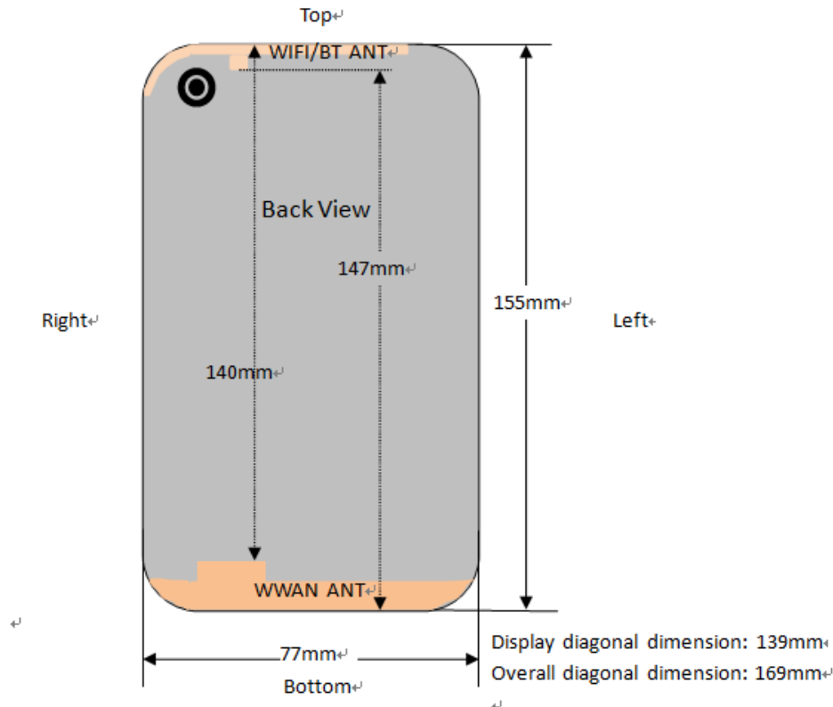
Fig.14.1 EUT Antenna Locations
