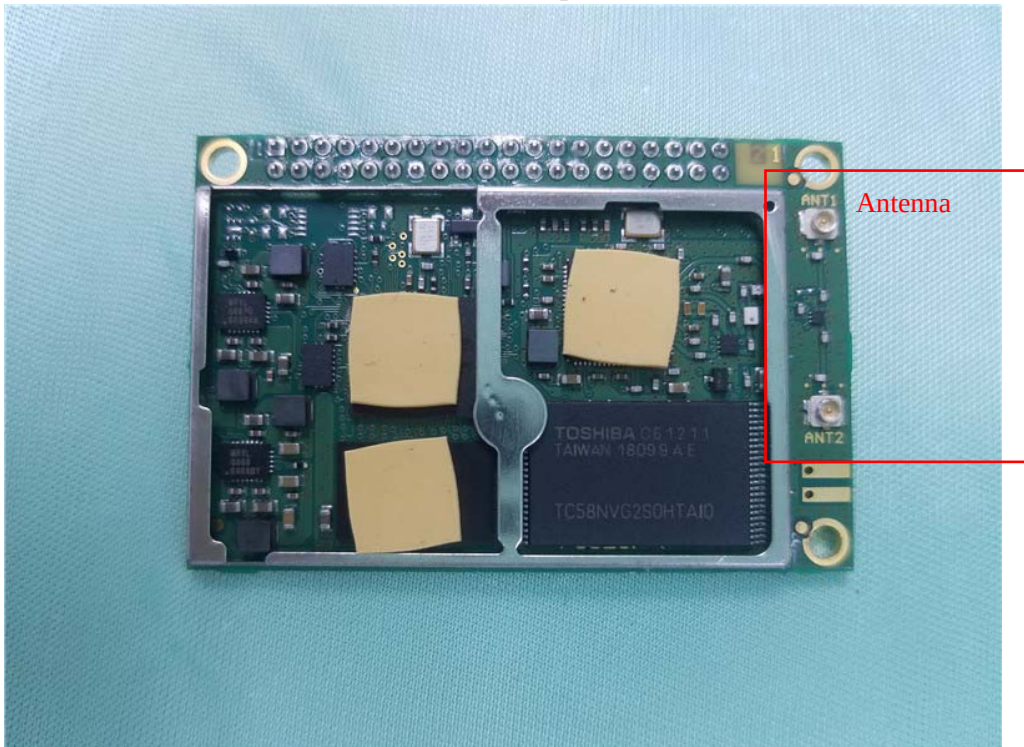
Inner Circuit Top View
