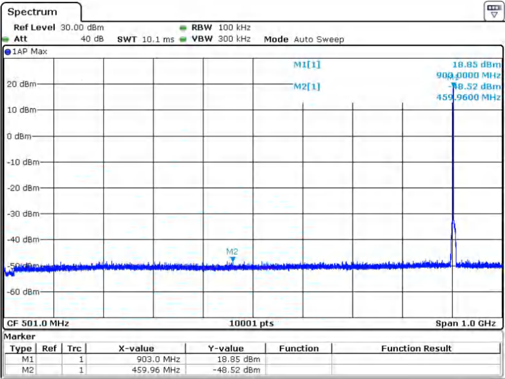
TX Frequency 903.0MHz _ 1M~1GHz
