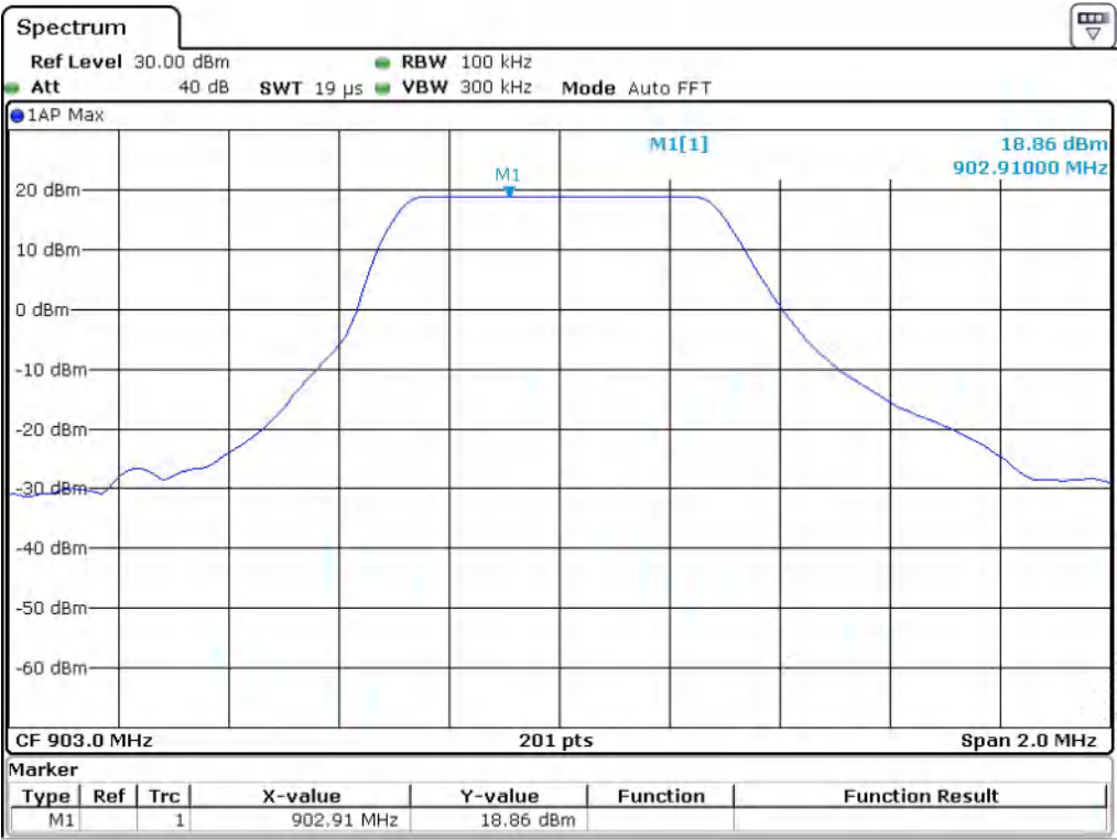
TX Frequency 903.0MHz _ Reference
