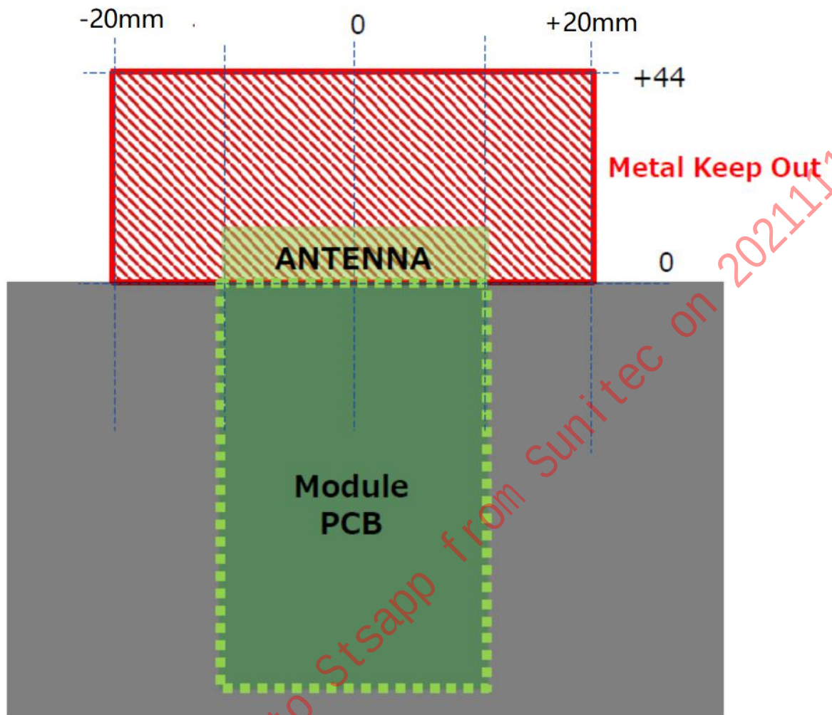
Figure 7.3-3 Recommended PWB footprint of the BMS002 module
