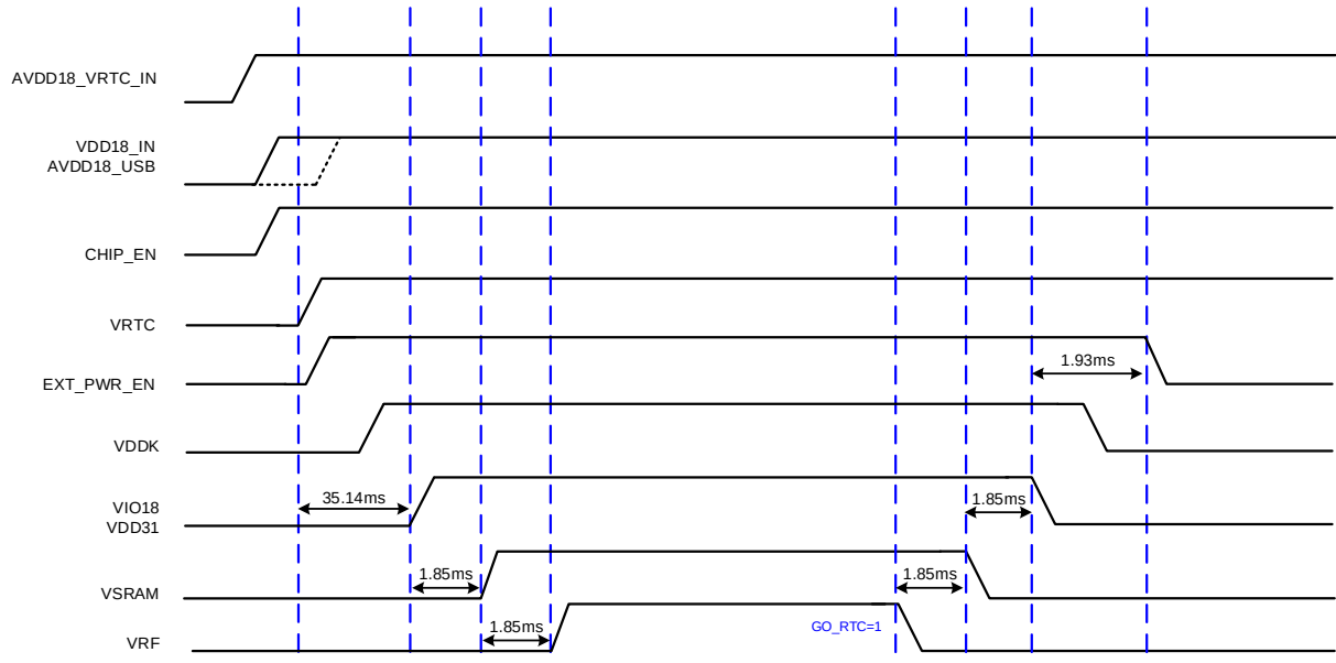
Figure 3.2-1 Power-on/off control sequence by charger plug-in
