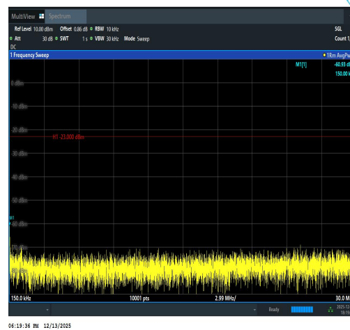
Band5-10MHz-16QAM-20525-1RB#49-0.15~30-
