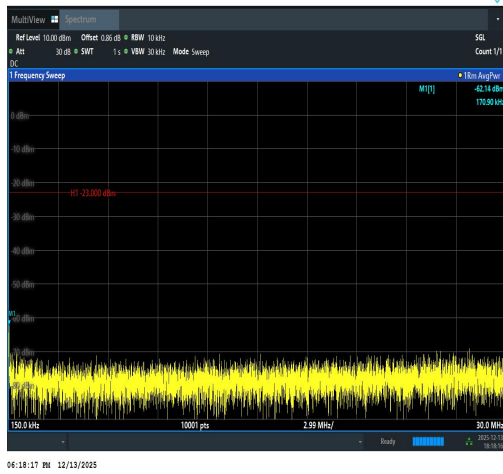
Band5-10MHz-16QAM-20525-1RB#0-0.15~30-P ASS
