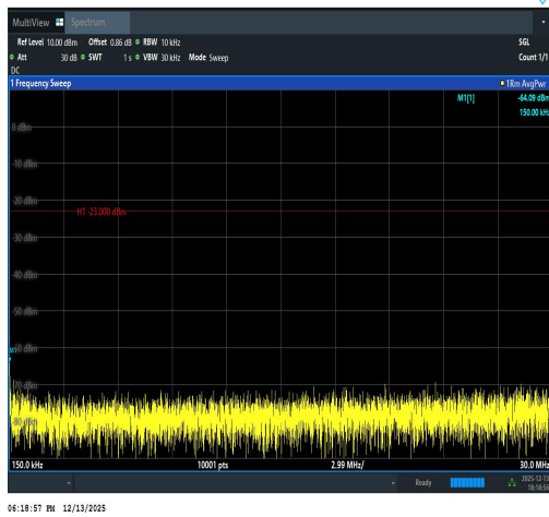
Band5-10MHz-QPSK-20525-1RB#49-0.15~30-P ASS
