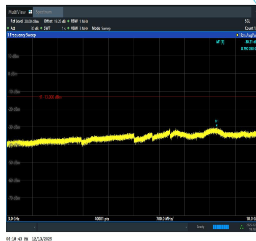
Band5-10MHz-16QAM-20525-1RB#0-3000~100 00-PASS
