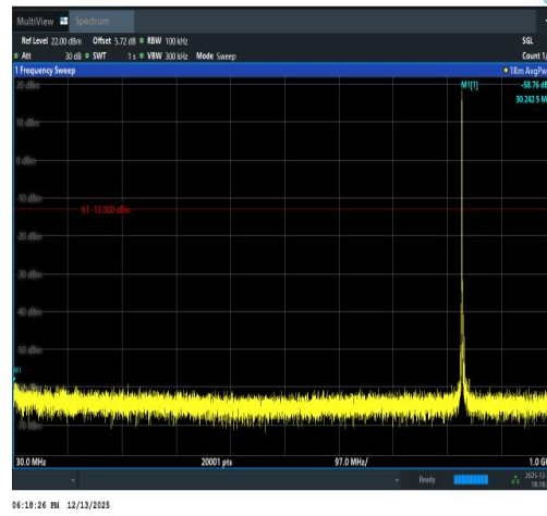
Band5-10MHz-16QAM-20525-1RB#0-30~1000-P ASS
