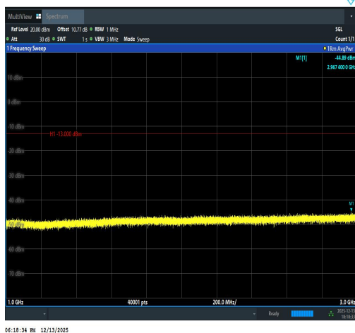
Band5-10MHz-16QAM-20525-1RB#0-1000~300 0-PASS
