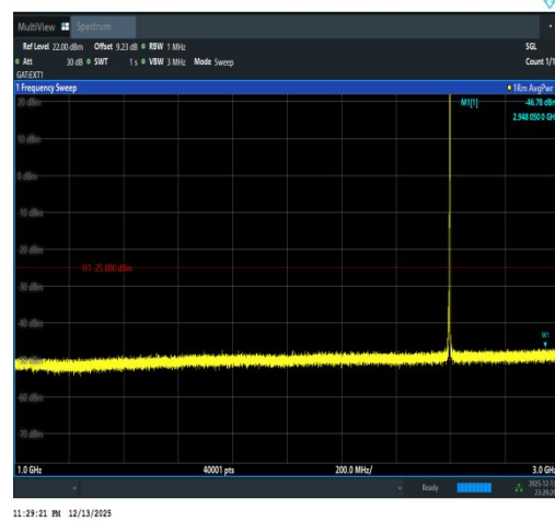
Band41(2535-2655)-5MHz-16QAM-40640-1RB# 24-1000~3000-PASS
