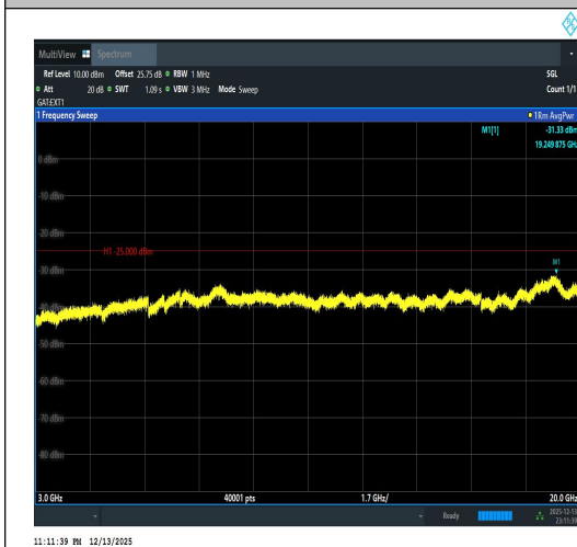
Band41(2535-2655)-5MHz-QPSK-40065-1RB#2 4-3000~20000-PASS
