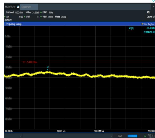
Band41(2535-2655)-5MHz-QPSK-40640-1RB#2 4-20000~27000-PASS
