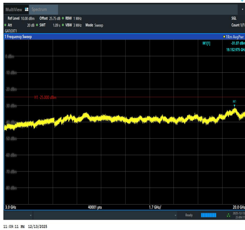
Band41(2535-2655)-5MHz-16QAM-40065-1RB# 0-3000~20000-PASS
