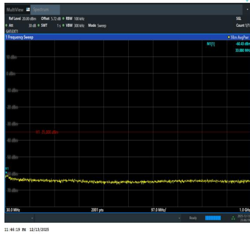
Band41(2535-2655)-5MHz-QPSK-41215-25RB# 0-30~1000-PASS
