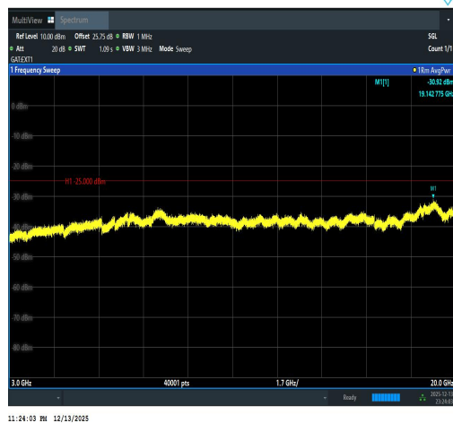
Band41(2535-2655)-5MHz-16QAM-40640-1RB# 0-3000~20000-PASS
