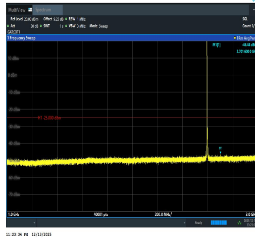
Band41(2535-2655)-5MHz-16QAM-40640-1RB# 0-1000~3000-PASS
