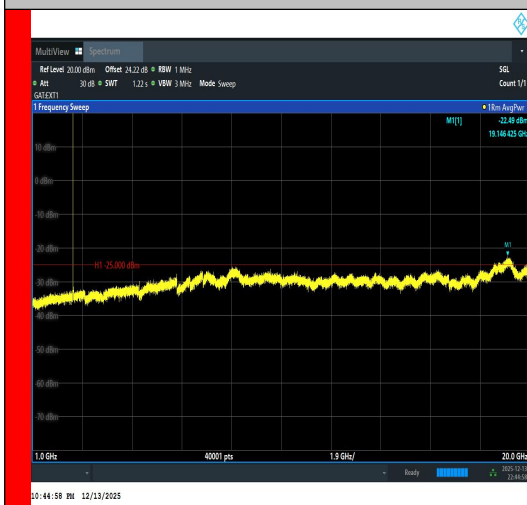
Band41(2535-2655)-5MHz-16QAM-40065-1RB# 24-1000~20000-FAIL
