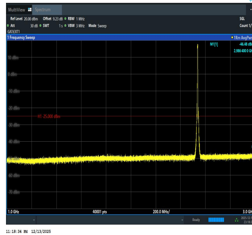
Band41(2535-2655)-5MHz-16QAM-40065-25RB #0-1000~3000-PASS
