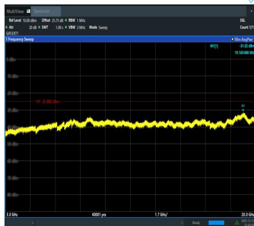
Band41(2535-2655)-5MHz-QPSK-40640-1RB#2 4-3000~20000-PASS
