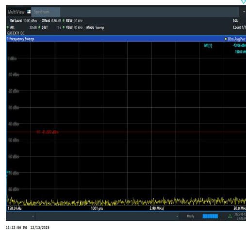
Band41(2535-2655)-5MHz-16QAM-40640-1RB#
