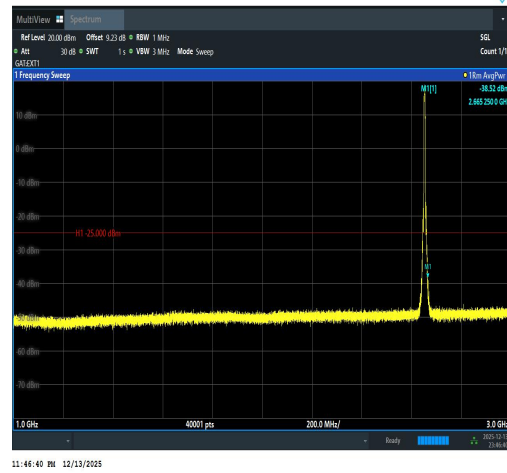
Band41(2535-2655)-5MHz-QPSK-41215-25RB# 0-1000~3000-PASS
