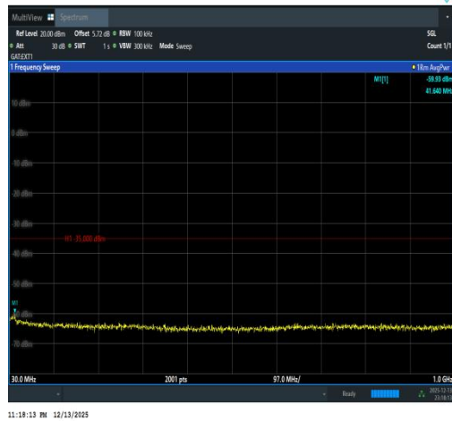
Band41(2535-2655)-5MHz-16QAM-40065-25RB #0-30~1000-PASS
