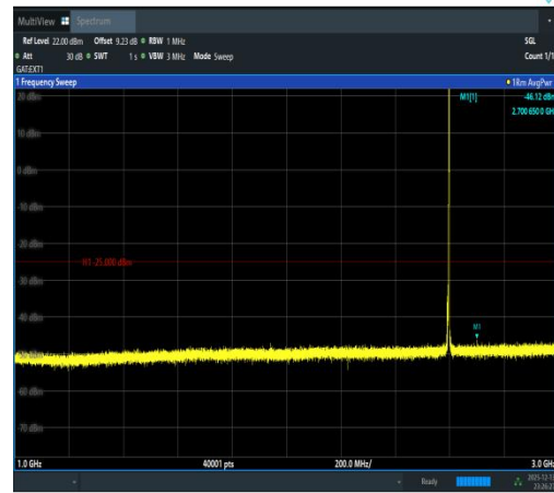
Band41(2535-2655)-5MHz-QPSK-40640-1RB#2 4-1000~3000-PASS
