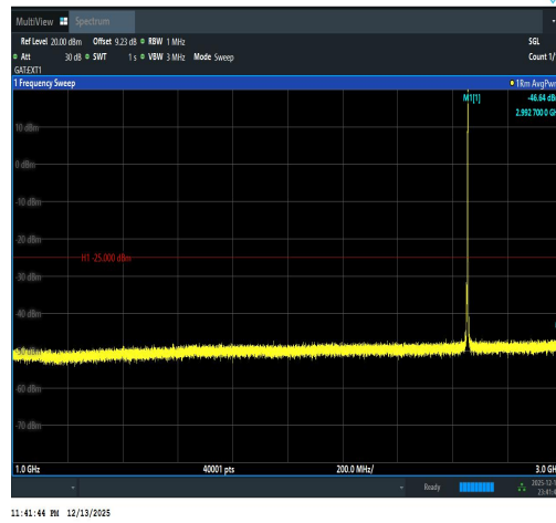
Band41(2535-2655)-5MHz-QPSK-41215-1RB#2 4-1000~3000-PASS
