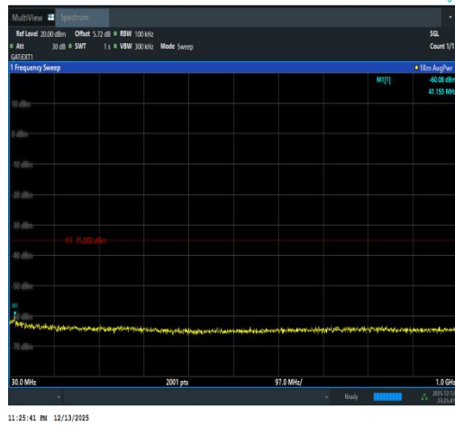
Band41(2535-2655)-5MHz-QPSK-40640-1RB#2 4-30~1000-PASS
