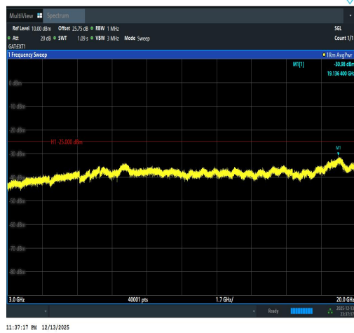
Band41(2535-2655)-5MHz-QPSK-41215-1RB#0-3000~20000-PASS
