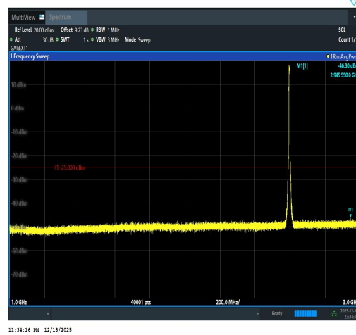
Band41(2535-2655)-5MHz-16QAM-40640-25RB #0-1000~3000-PASS
