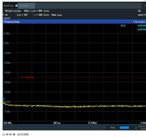
Band41(2535-2655)-5MHz-QPSK-41215-1RB#0-30~1000-PASS
