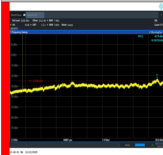
Band41(2535-2655)-5MHz-QPSK-40065-1RB#2 4-1000~20000-FAIL
