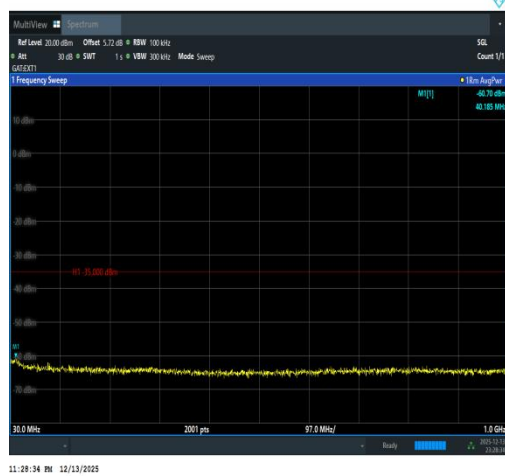
Band41(2535-2655)-5MHz-16QAM-40640-1RB# 24-30~1000-PASS
