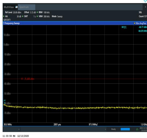
Band41(2535-2655)-5MHz-16QAM-40640-25RB #0-30~1000-PASS
