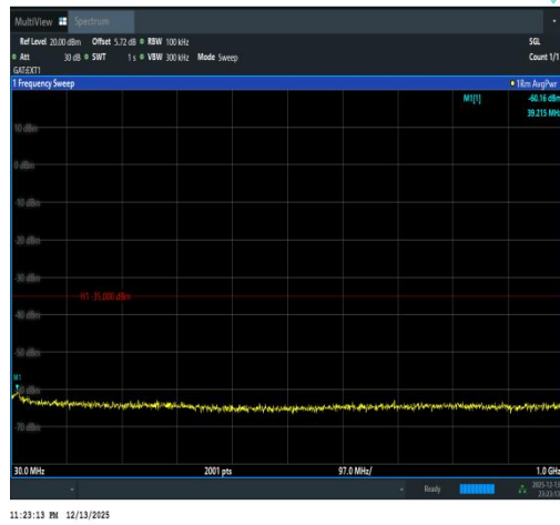
Band41(2535-2655)-5MHz-16QAM-40640-1RB# 0-30~1000-PASS
