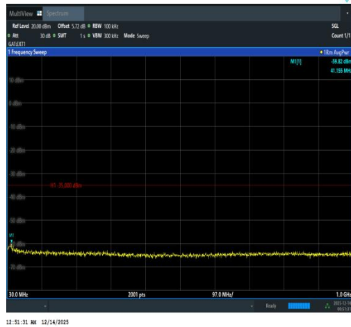
Band41(2535-2655)-10MHz-QPSK-40090-50RB #0-30~1000-PASS
