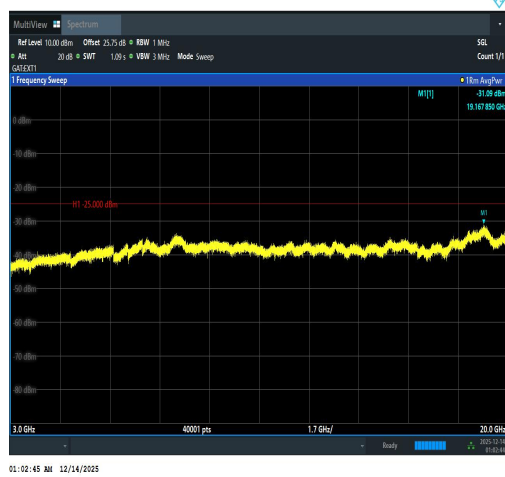
Band41(2535-2655)-10MHz-QPSK-40640-1RB# 49-3000~20000-PASS
