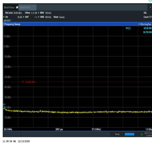
Band41(2535-2655)-5MHz-16QAM-41215-1RB# 0-30~1000-PASS
