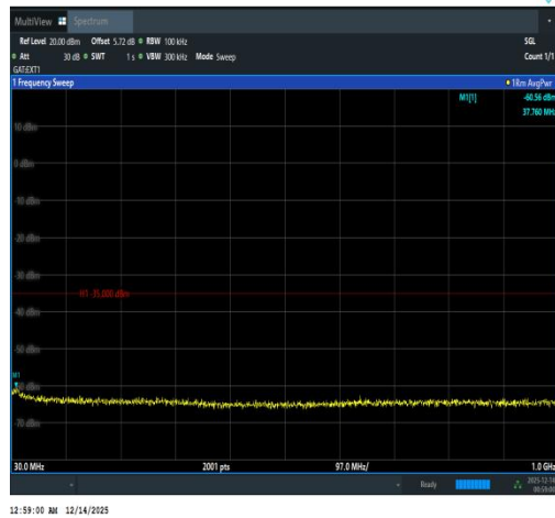
Band41(2535-2655)-10MHz-16QAM-40640-1RB #0-30~1000-PASS
