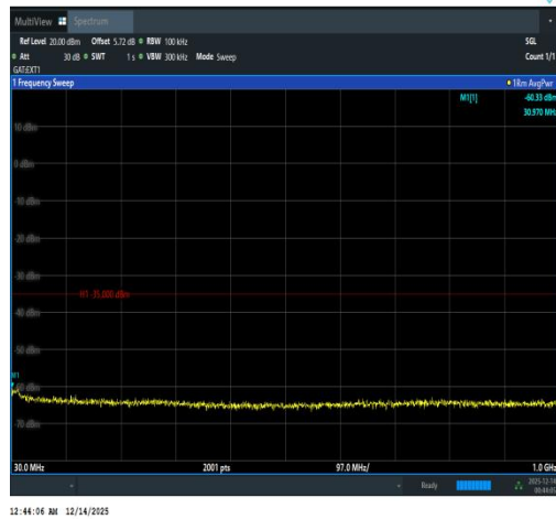
Band41(2535-2655)-10MHz-16QAM-40090-1RB #0-30~1000-PASS
