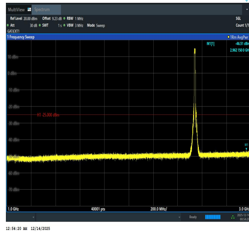
Band41(2535-2655)-10MHz-16QAM-40090-50R B#0-1000~3000-PASS
