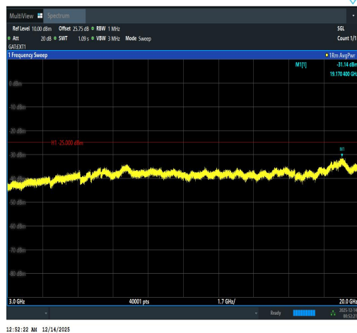
Band41(2535-2655)-10MHz-QPSK-40090-50RB #0-3000~20000-PASS
