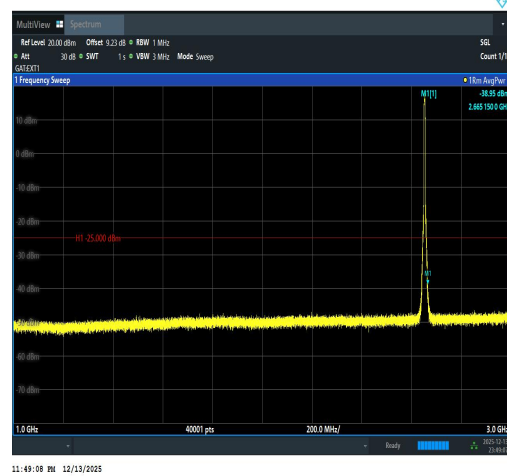
Band41(2535-2655)-5MHz-16QAM-41215-25RB #0-1000~3000-PASS
