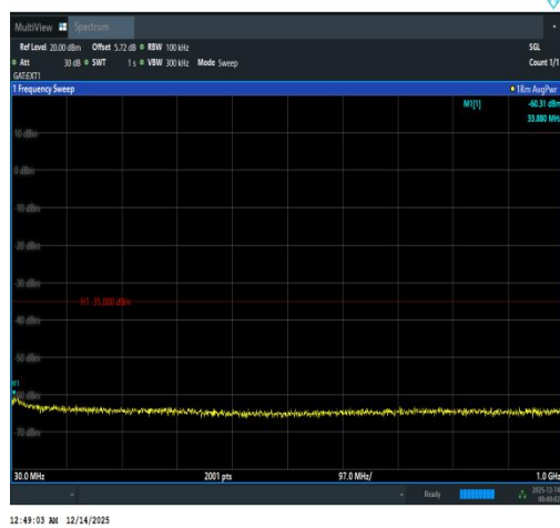
Band41(2535-2655)-10MHz-16QAM-40090-1RB #49-30~1000-PASS
