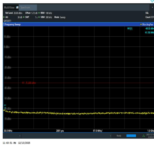
Band41(2535-2655)-5MHz-16QAM-41215-1RB# 24-30~1000-PASS
