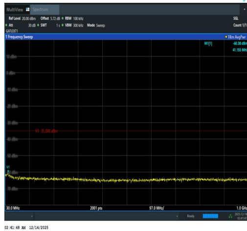
Band41(2535-2655)-15MHz-QPSK-41165-75RB #0-30~1000-PASS
