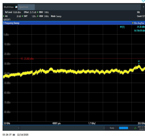
Band41(2535-2655)-20MHz-QPSK-40140-1RB# 99-3000~20000-PASS
