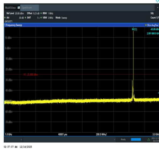
Band41(2535-2655)-15MHz-QPSK-41165-1RB# 74-1000~3000-PASS
