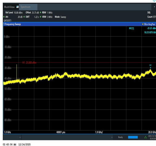
Band41(2535-2655)-15MHz-QPSK-41165-75RB #0-1000~20000-PASS
