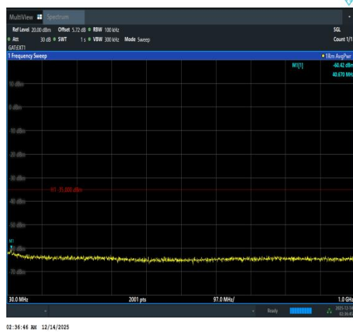
Band41(2535-2655)-15MHz-QPSK-41165-1RB# 74-30~1000-PASS
