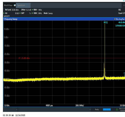
Band41(2535-2655)-15MHz-16QAM-41165-1RB #74-1000~3000-PASS
