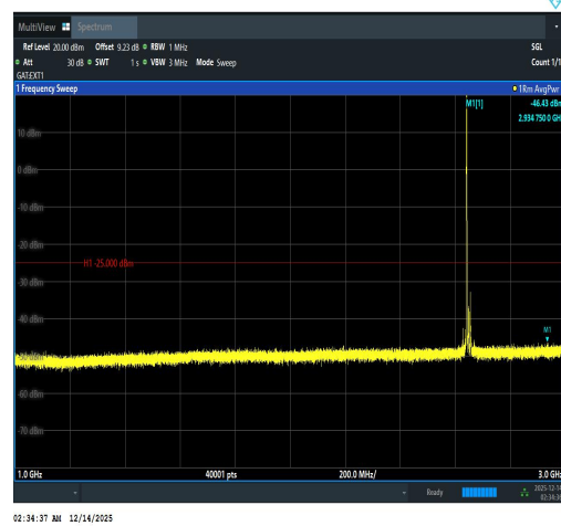
Band41(2535-2655)-15MHz-16QAM-41165-1RB #0-1000~3000-PASS
