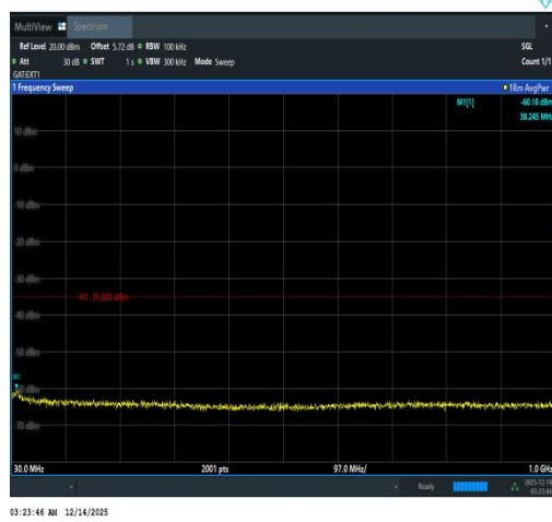
Band41(2535-2655)-20MHz-QPSK-40140-1RB# 99-30~1000-PASS
