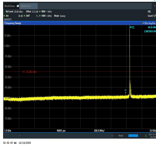
Band41(2535-2655)-15MHz-QPSK-41165-1RB# 0-1000~3000-PASS
