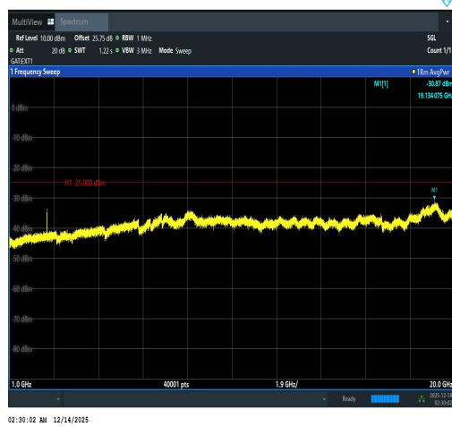
Band41(2535-2655)-15MHz-16QAM-40640-75R B#0-1000~20000-PASS
