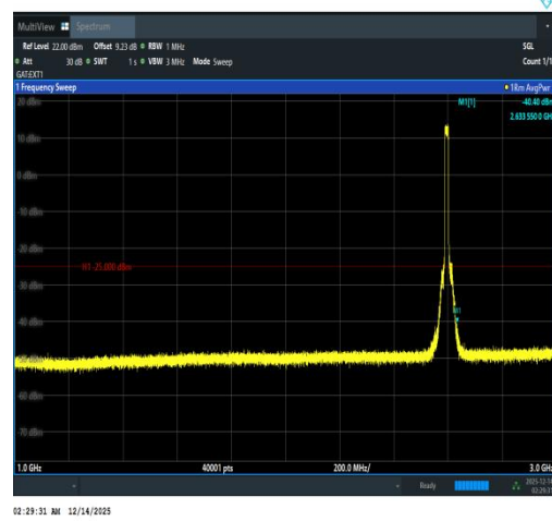
Band41(2535-2655)-15MHz-16QAM-40640-75R B#0-1000~3000-PASS
