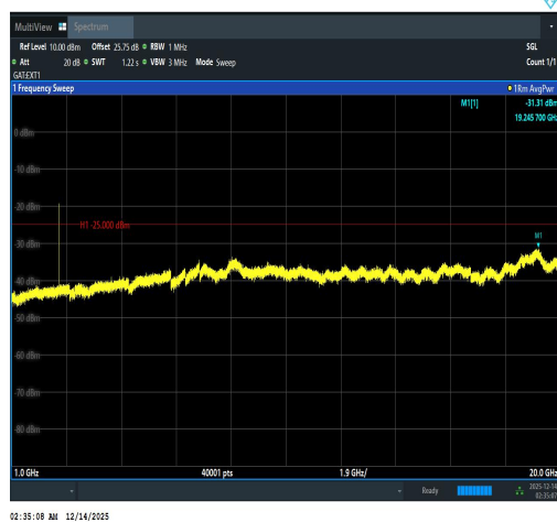
Band41(2535-2655)-15MHz-16QAM-41165-1RB #0-1000~20000-PASS
