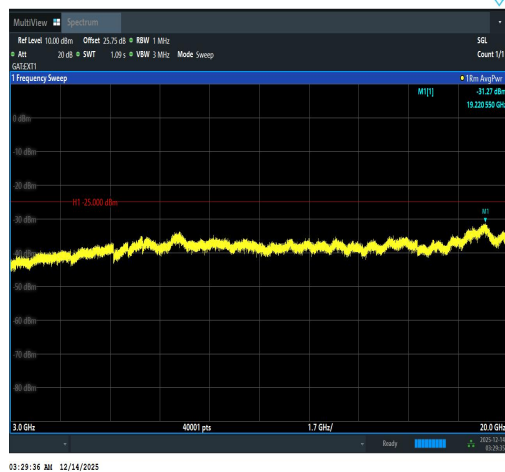
Band41(2535-2655)-20MHz-QPSK-40140-100R B#0-3000~20000-PASS
