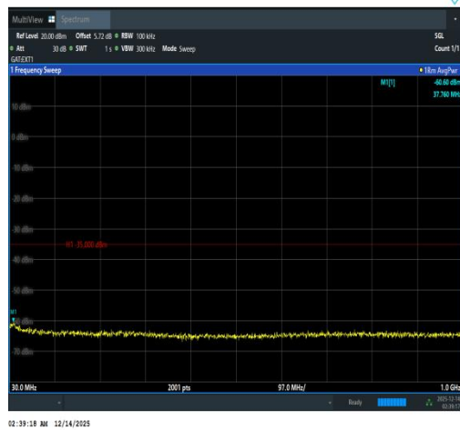
Band41(2535-2655)-15MHz-16QAM-41165-1RB #74-30~1000-PASS
