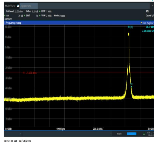
Band41(2535-2655)-15MHz-QPSK-41165-75RB #0-1000~3000-PASS
