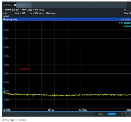
Band41(2535-2655)-20MHz-QPSK-40140-1RB# 0-30~1000-PASS
