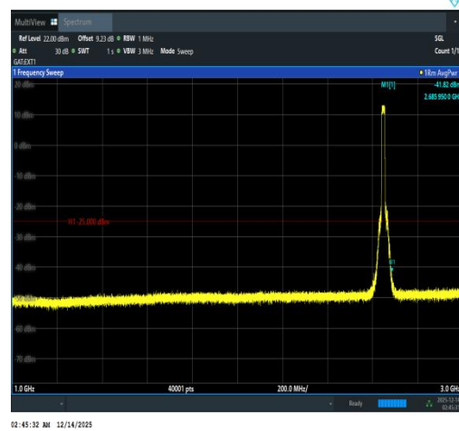
Band41(2535-2655)-15MHz-16QAM-41165-75R B#0-1000~3000-PASS
