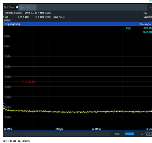
Band41(2535-2655)-15MHz-16QAM-41165-75R B#0-30~1000-PASS
