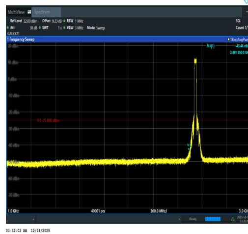
Band41(2535-2655)-20MHz-16QAM-40140-100 RB#0-1000~3000-PASS
