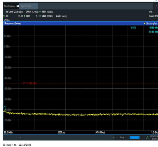
Band41(2535-2655)-20MHz-16QAM-40140-1RB #0-30~1000-PASS
