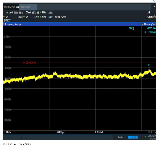
Band41(2535-2655)-20MHz-16QAM-40140-1RB #99-3000~20000-PASS
