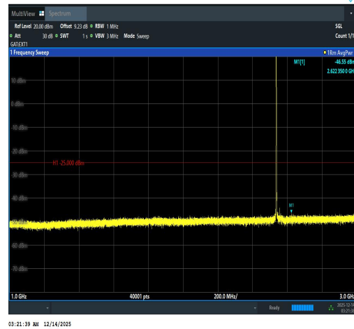
Band41(2535-2655)-20MHz-16QAM-40140-1RB #0-1000~3000-PASS
