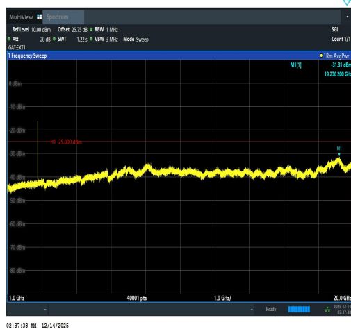
Band41(2535-2655)-15MHz-QPSK-41165-1RB# 74-1000~20000-PASS
