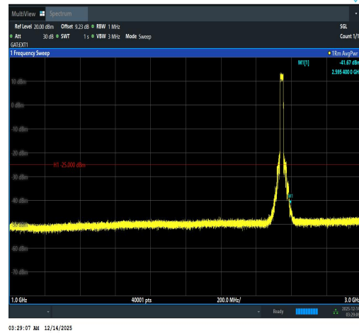
Band41(2535-2655)-20MHz-QPSK-40140-100R B#0-1000~3000-PASS
