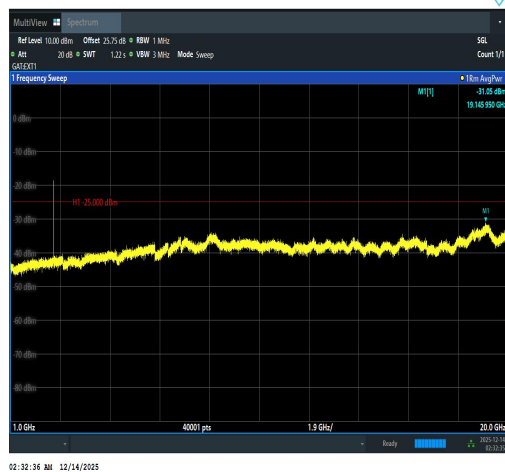
Band41(2535-2655)-15MHz-QPSK-41165-1RB# 0-1000~20000-PASS
