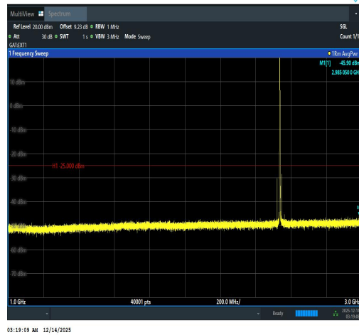
Band41(2535-2655)-20MHz-QPSK-40140-1RB# 0-1000~3000-PASS
