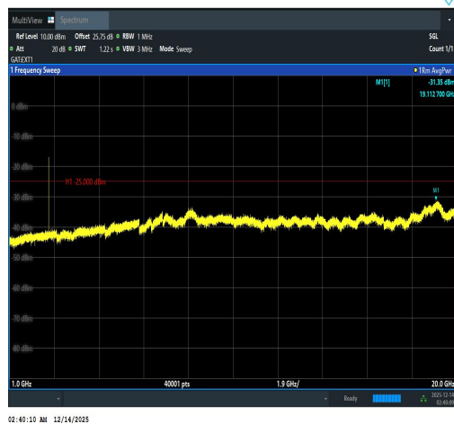
Band41(2535-2655)-15MHz-16QAM-41165-1RB #74-1000~20000-PASS
