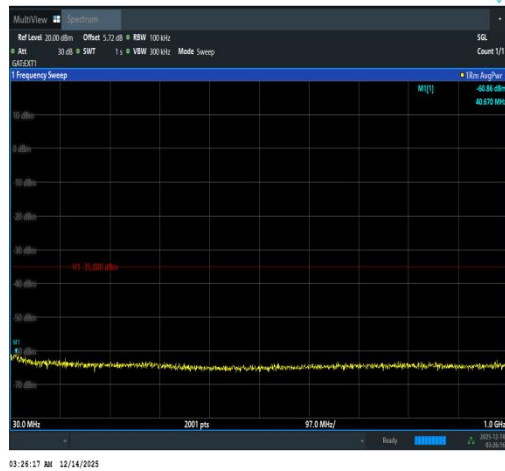
Band41(2535-2655)-20MHz-16QAM-40140-1RB #99-30~1000-PASS
