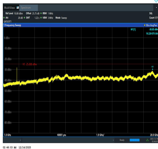
Band41(2535-2655)-15MHz-16QAM-41165-75R B#0-1000~20000-PASS
