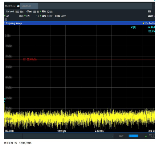
Band5-3MHz-16QAM-20415-1RB#14-0.15~30-P ASS
