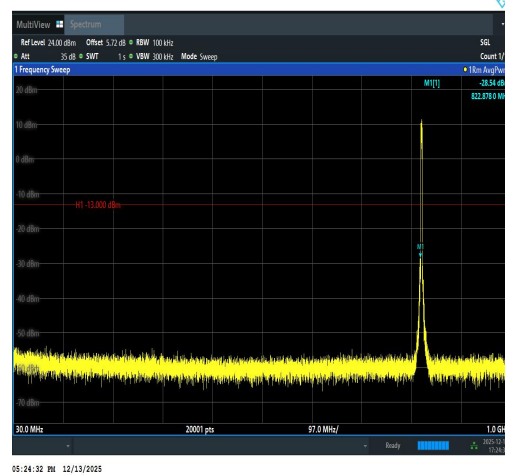
Band5-3MHz-16QAM-20415-15RB#0-30~1000-P ASS
