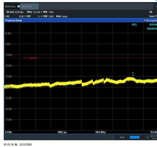
Band5-1.4MHz-16QAM-20643-1RB#0-3000~100 00-PASS
