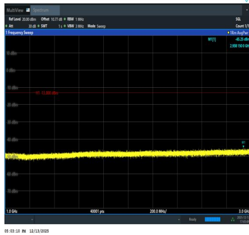
Band5-1.4MHz-16QAM-20643-1RB#0-1000~300 0-PASS
