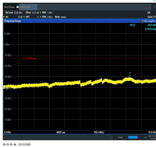
Band5-3MHz-16QAM-20415-1RB#14-3000~100 00-PASS
