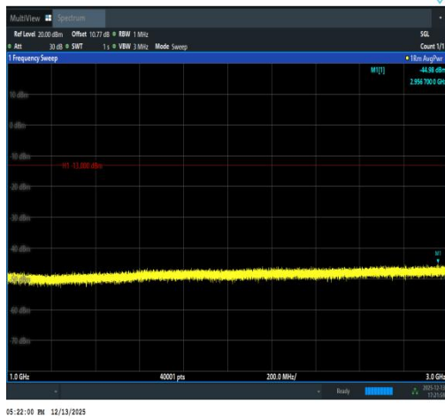
Band5-3MHz-16QAM-20415-1RB#0-1000~3000-PASS
