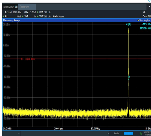
Band5-1.4MHz-QPSK-20643-6RB#0-30~1000-P ASS
