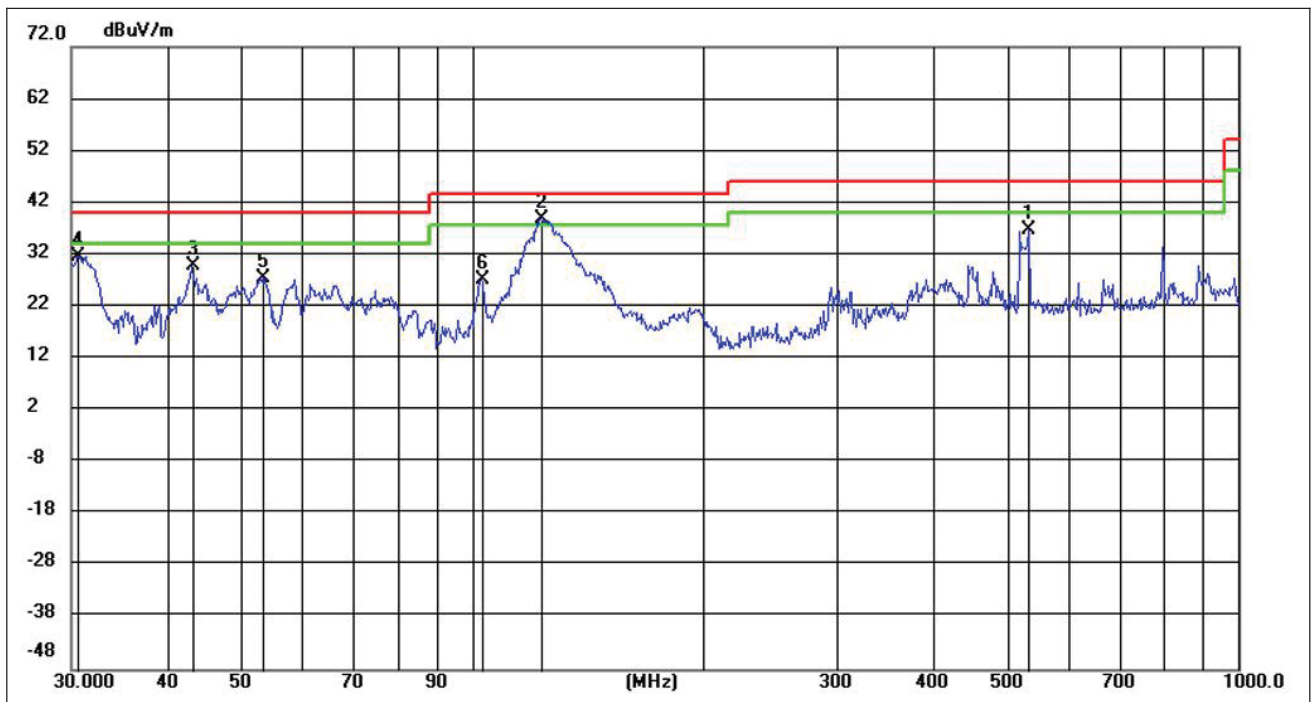
(Antenna Vertical, 30MHz to 1GHz)
