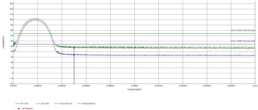
Plot for Channel 78
