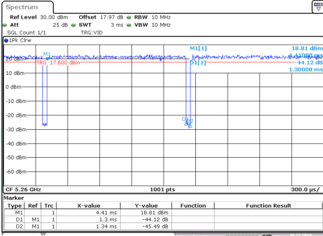
NTNV-11N20SISO-Ant1-5260
