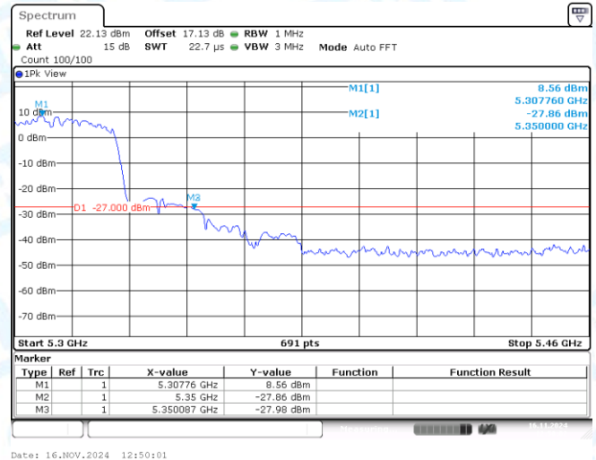
11N40SISO-Ant1-5310-PASS
