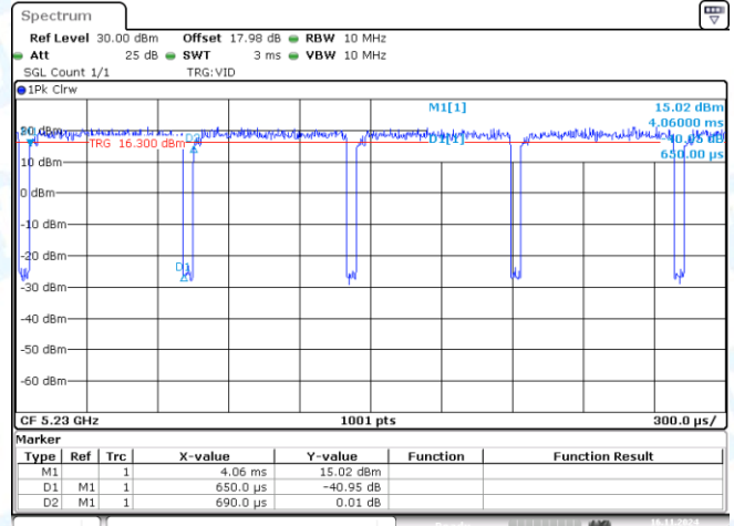
NTNV-11N40SISO-Ant1-5230
