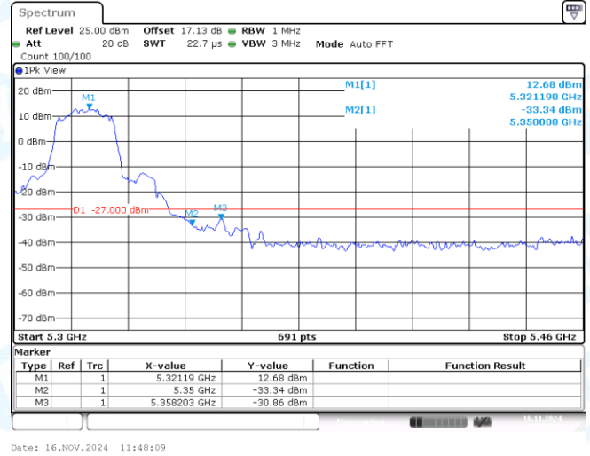
11A-Ant1-5320-PASS
