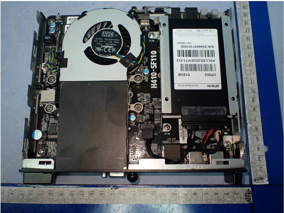
Figure 26 Case B Internal View
