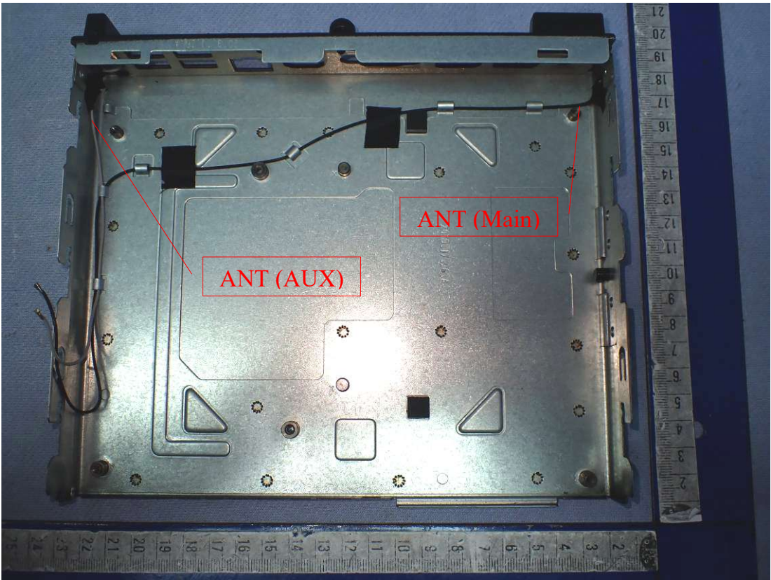
Figure 20 Case A Internal View
