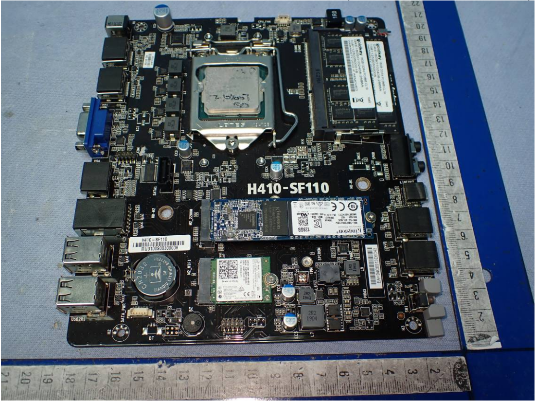
Figure 22 Case A Internal View (Mother Board, Front View)
