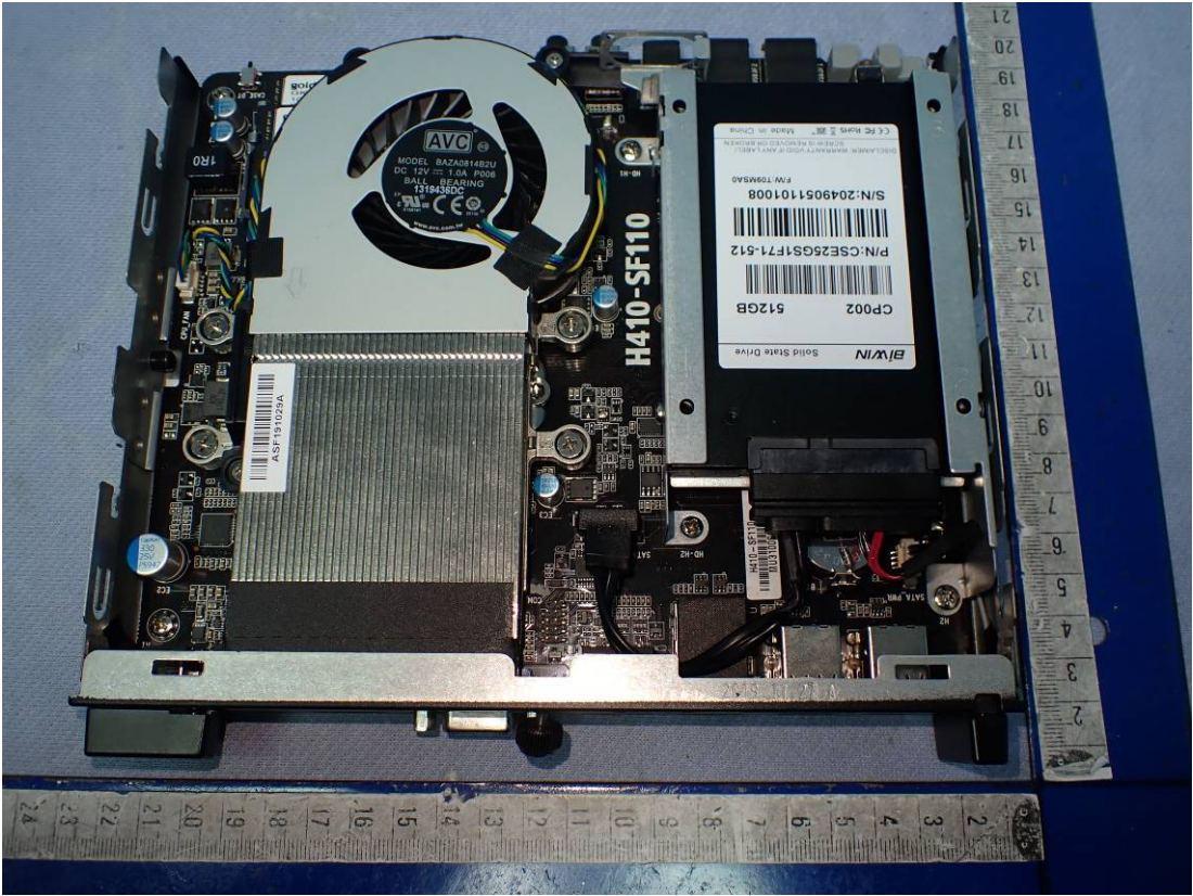
Figure 21 Case A Internal View
