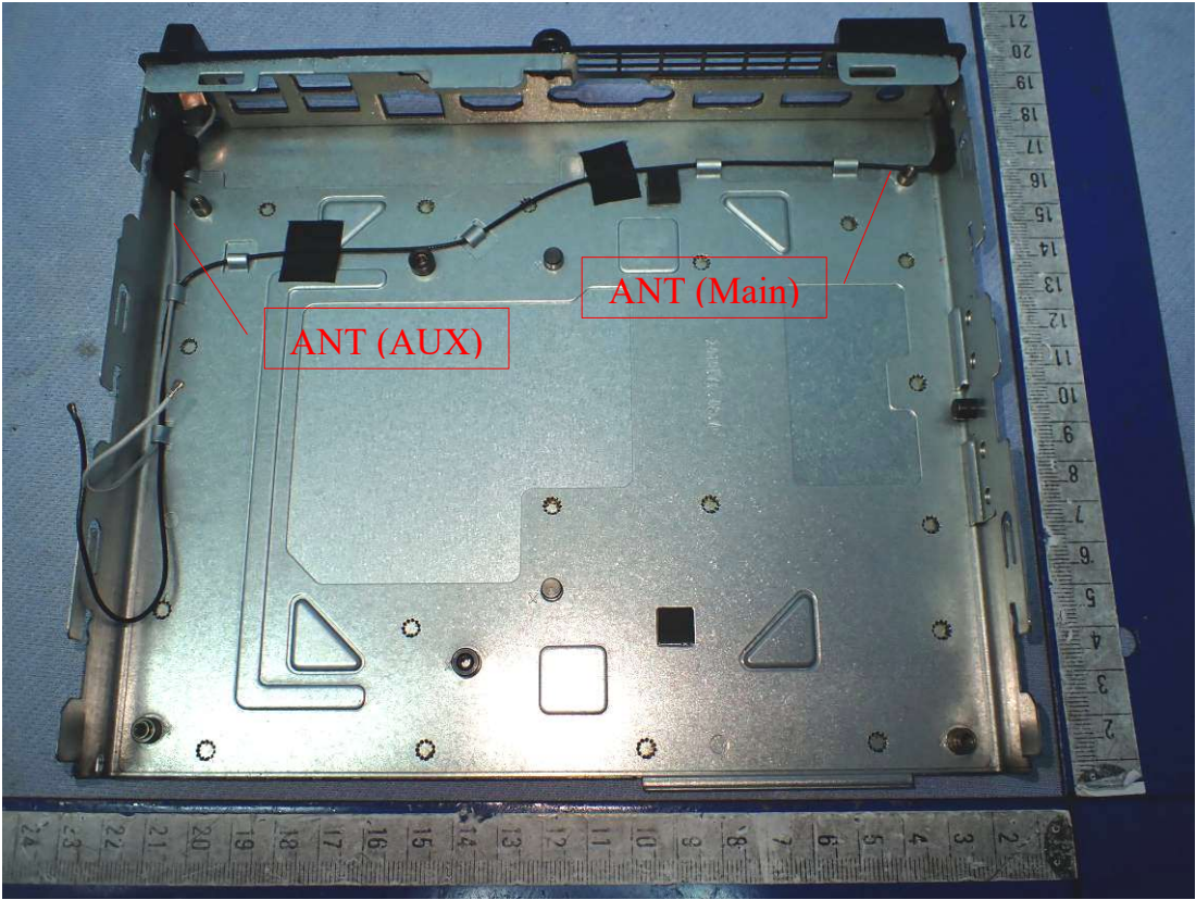
Figure 27 Case B Internal View
