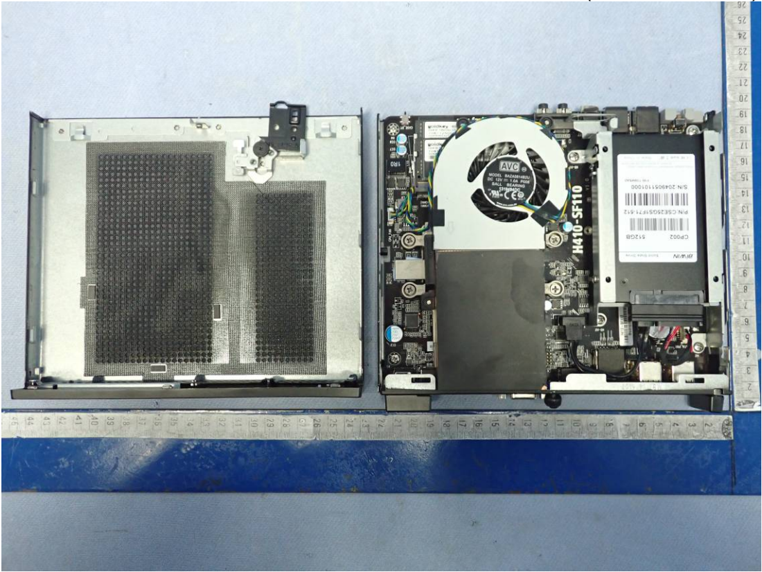
Figure 25 Case B Internal View (Removed Cover)
