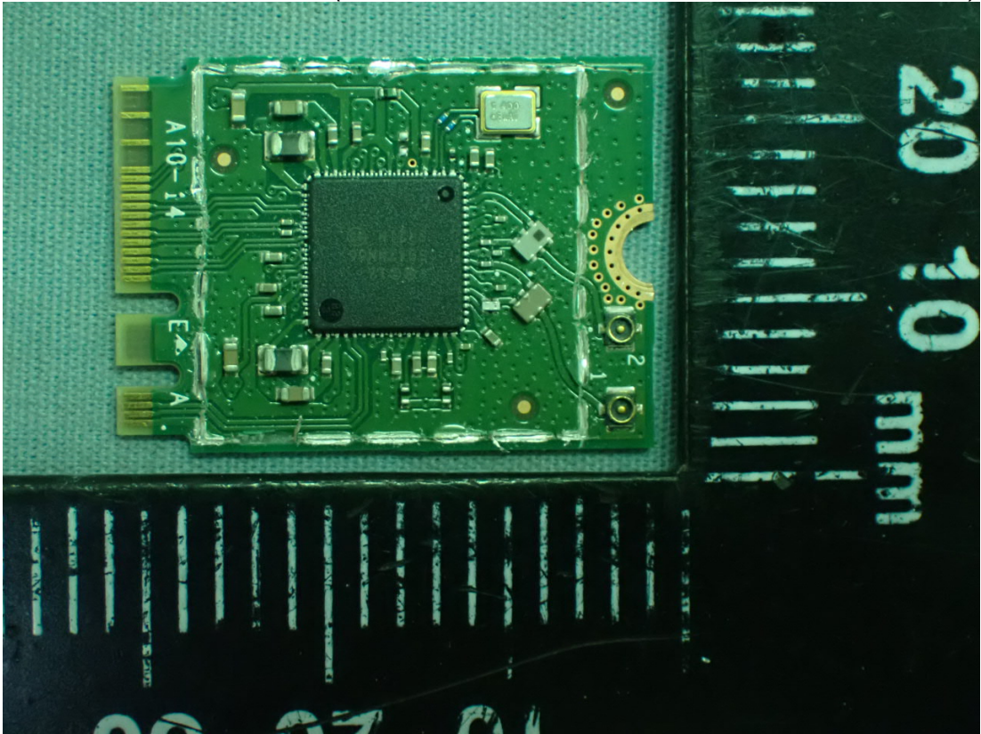
Figure 30 Internal View (WLAN Combo Card, Removed Cover, Front View)
