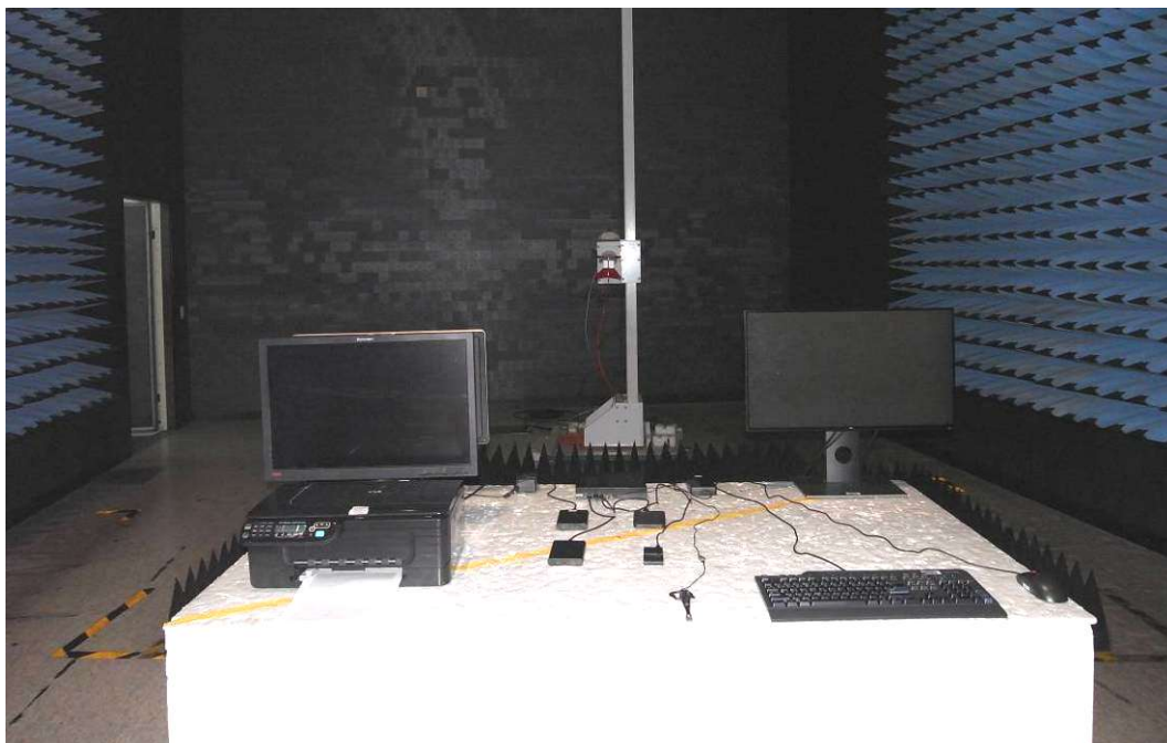
FRONT VIEW
