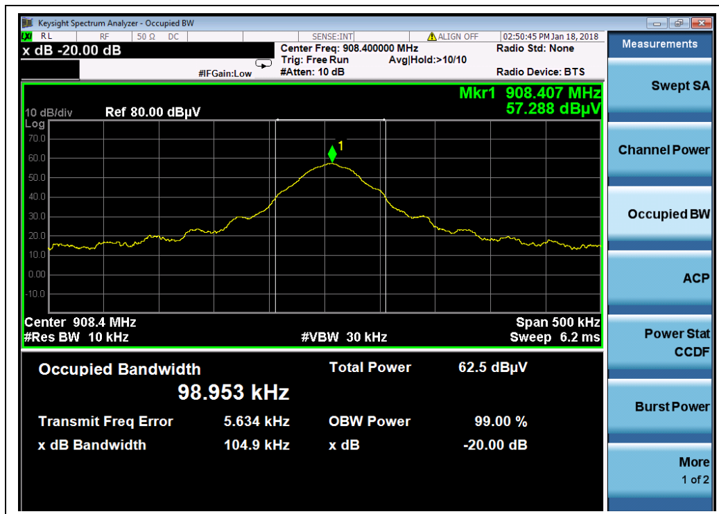
(Channel 1: 908.4MHz)
