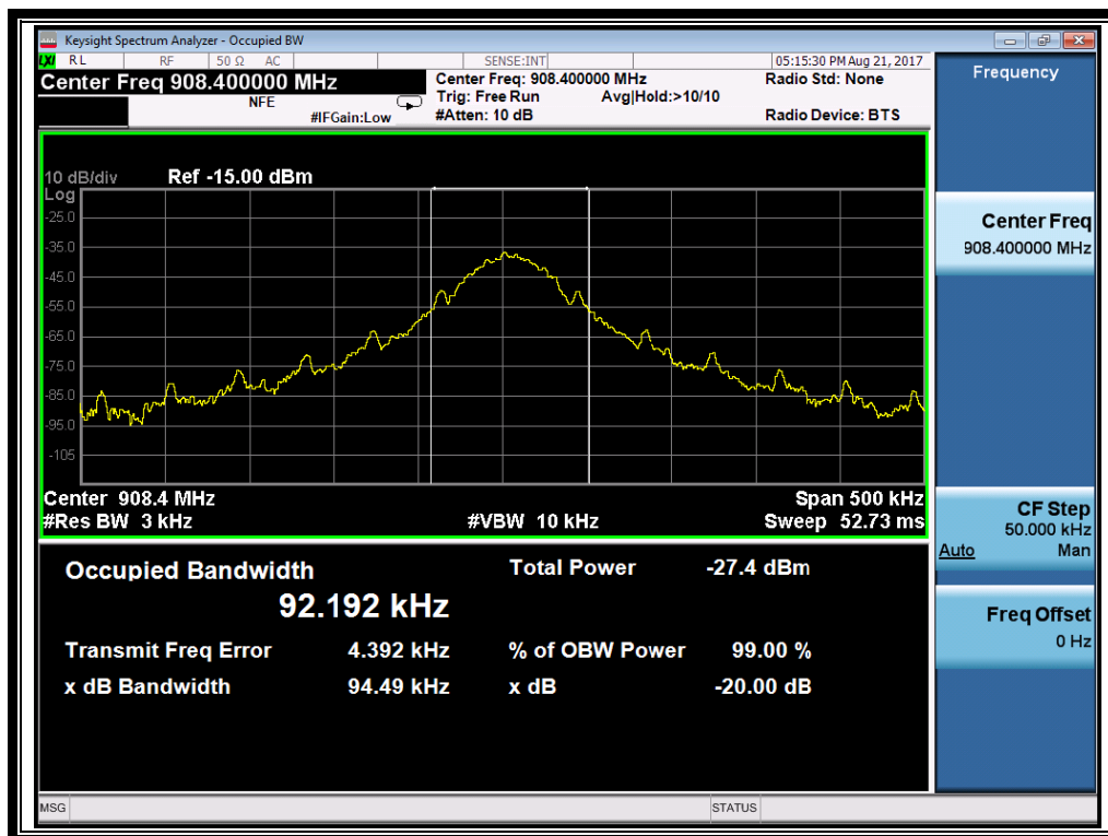
(Plot A, Channel 1: 908.4MHz)
