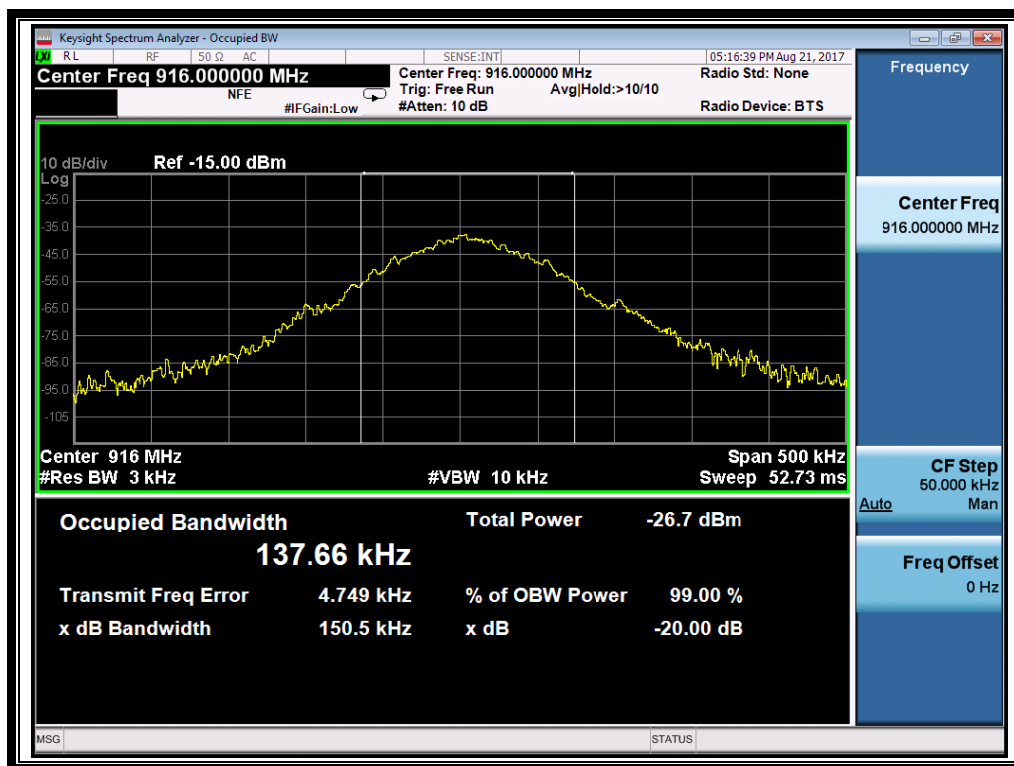
(Plot B, Channel 2: 916MHz)
