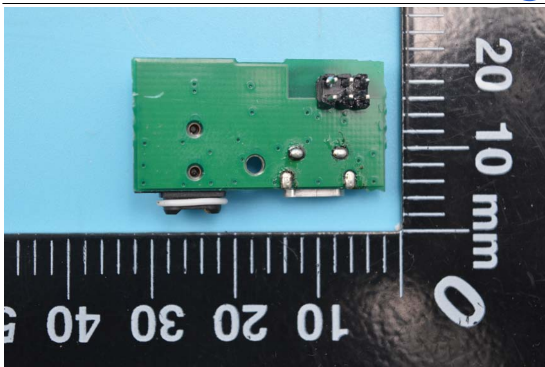
4. PCB antenna view
