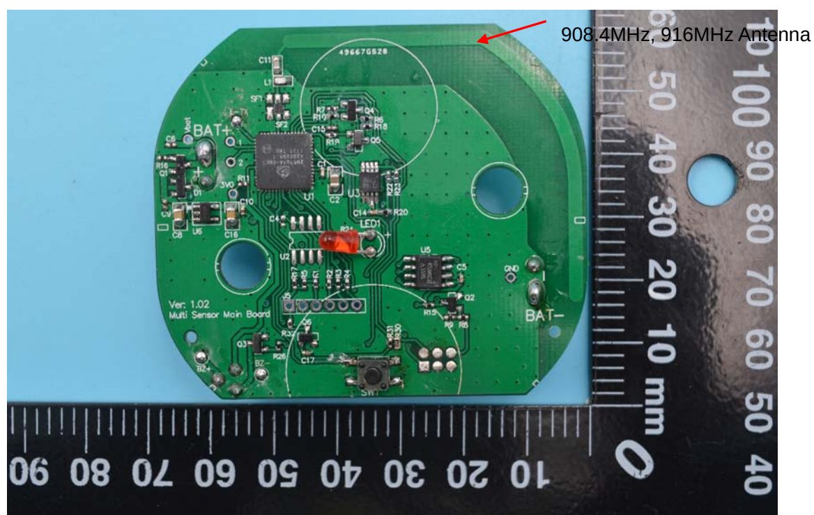
4. PCB antenna view
