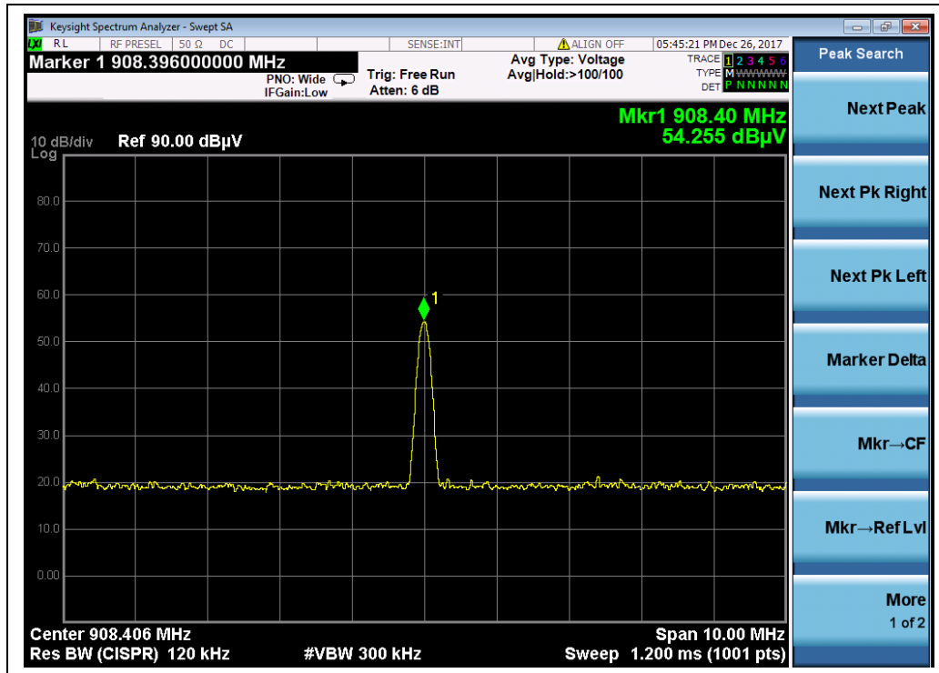
(Channel 1: 908.4MHz)
