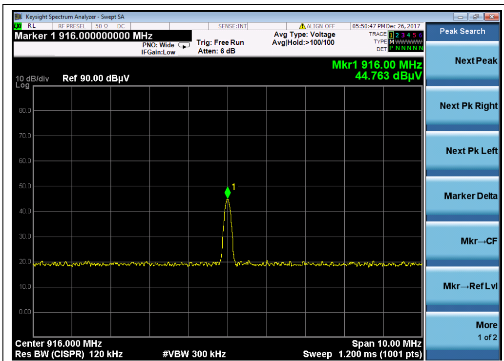
(Channel 2: 916.0 MHz)
