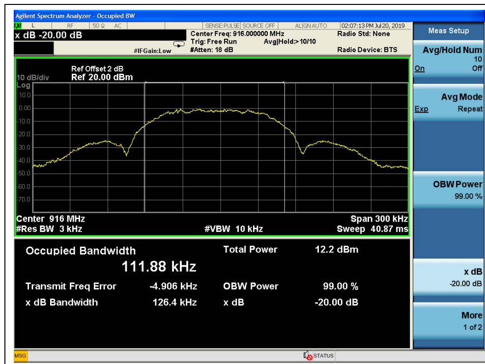
(Channel 2, 916.0 MHz)
