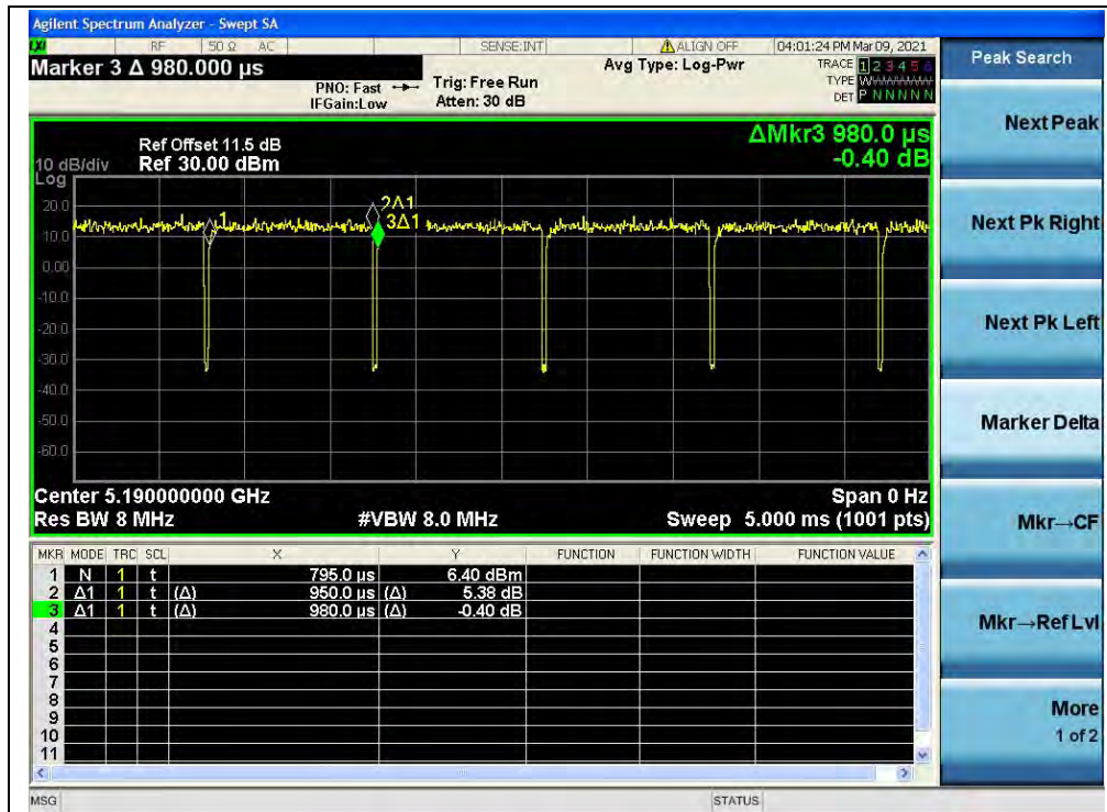
(CH38_5190MHz_802.11ac (VHT40))
