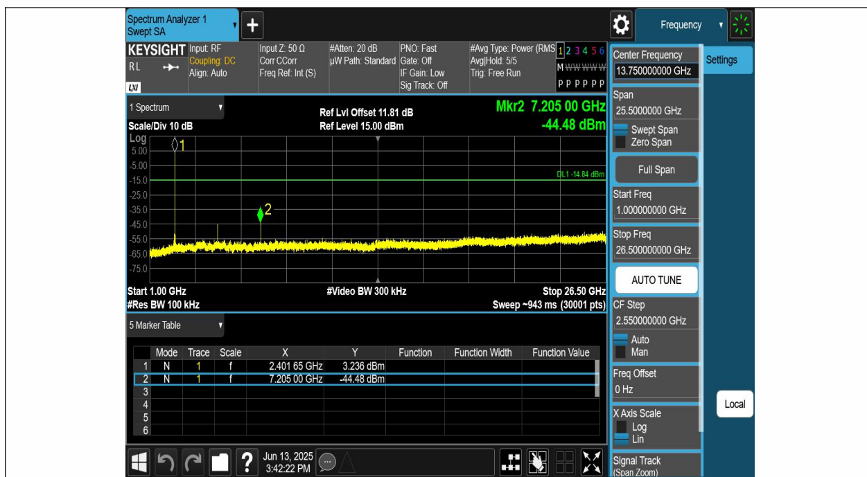
GFSK-Ant1-2402-1000~26500-PASS
