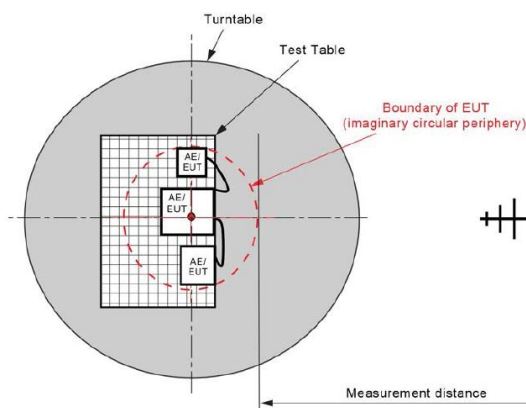
Figure C.1 – Measurement distance
