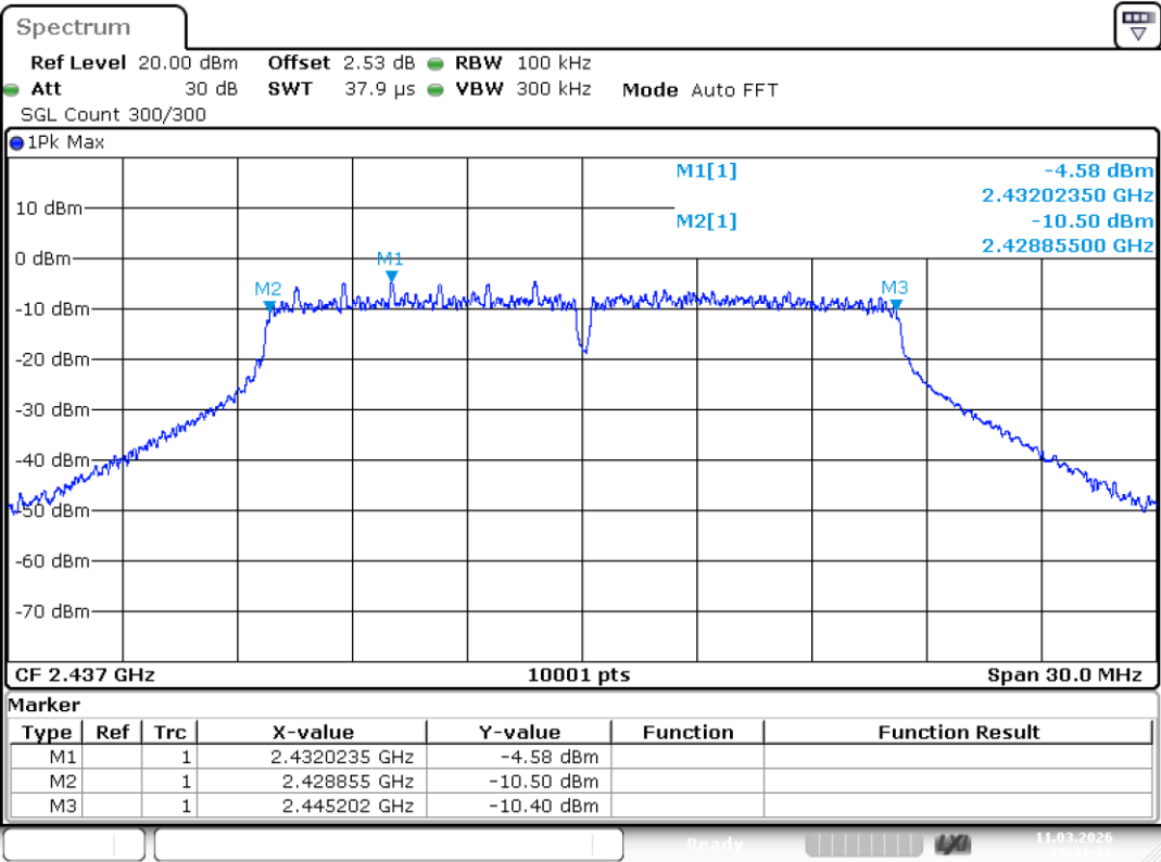
-6dB Bandwidth NVNT g 2437MHz Ant1
