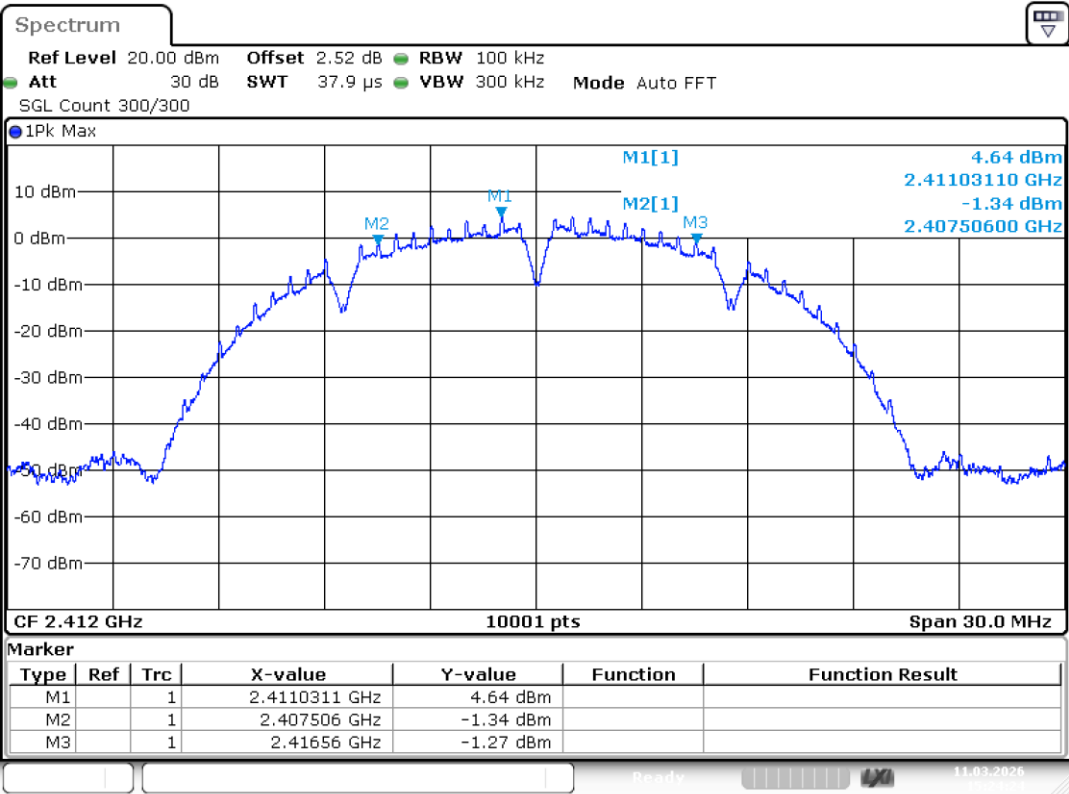
-6dB Bandwidth NVNT b 2412MHz Ant1
