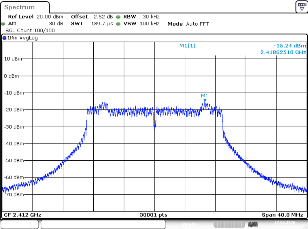
PSD NVNT n20 2412MHz Ant1
