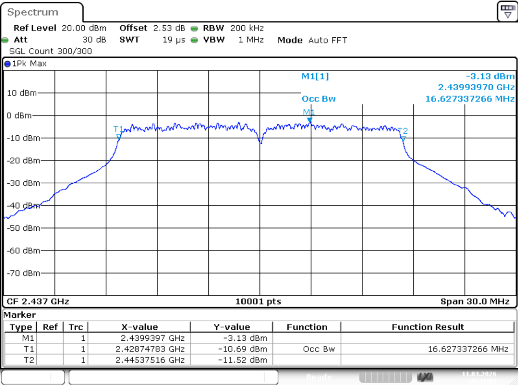
OBW NVNT g 2437MHz Ant1
