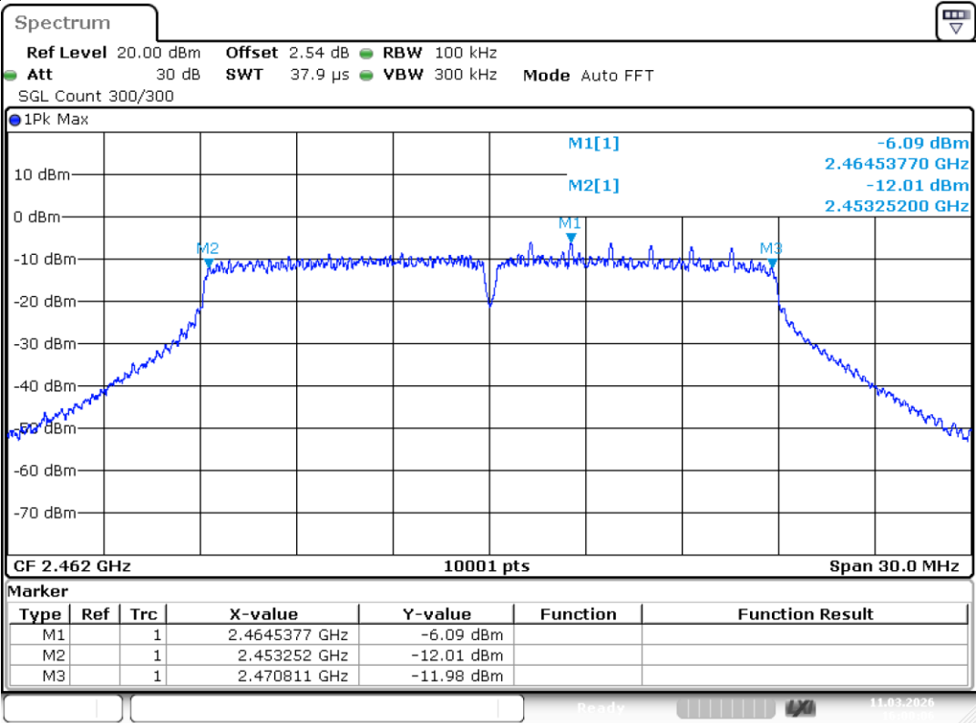
-6dB Bandwidth NVNT n20 2462MHz Ant1
