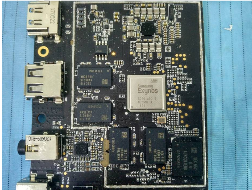
EUT – IC Mains View
