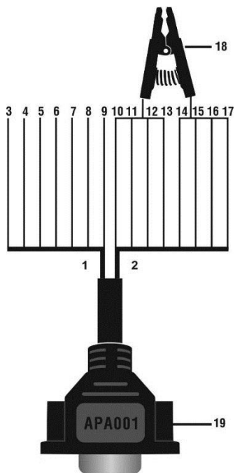
Figure 2-6 EEPROM Clamp Integrated MC9S12 Cable
