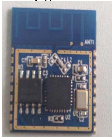
Photograph of Modularly approved WiFi board without shield
