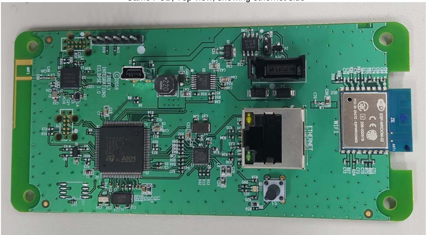
Same PCB; Top view, showing ethernet side
