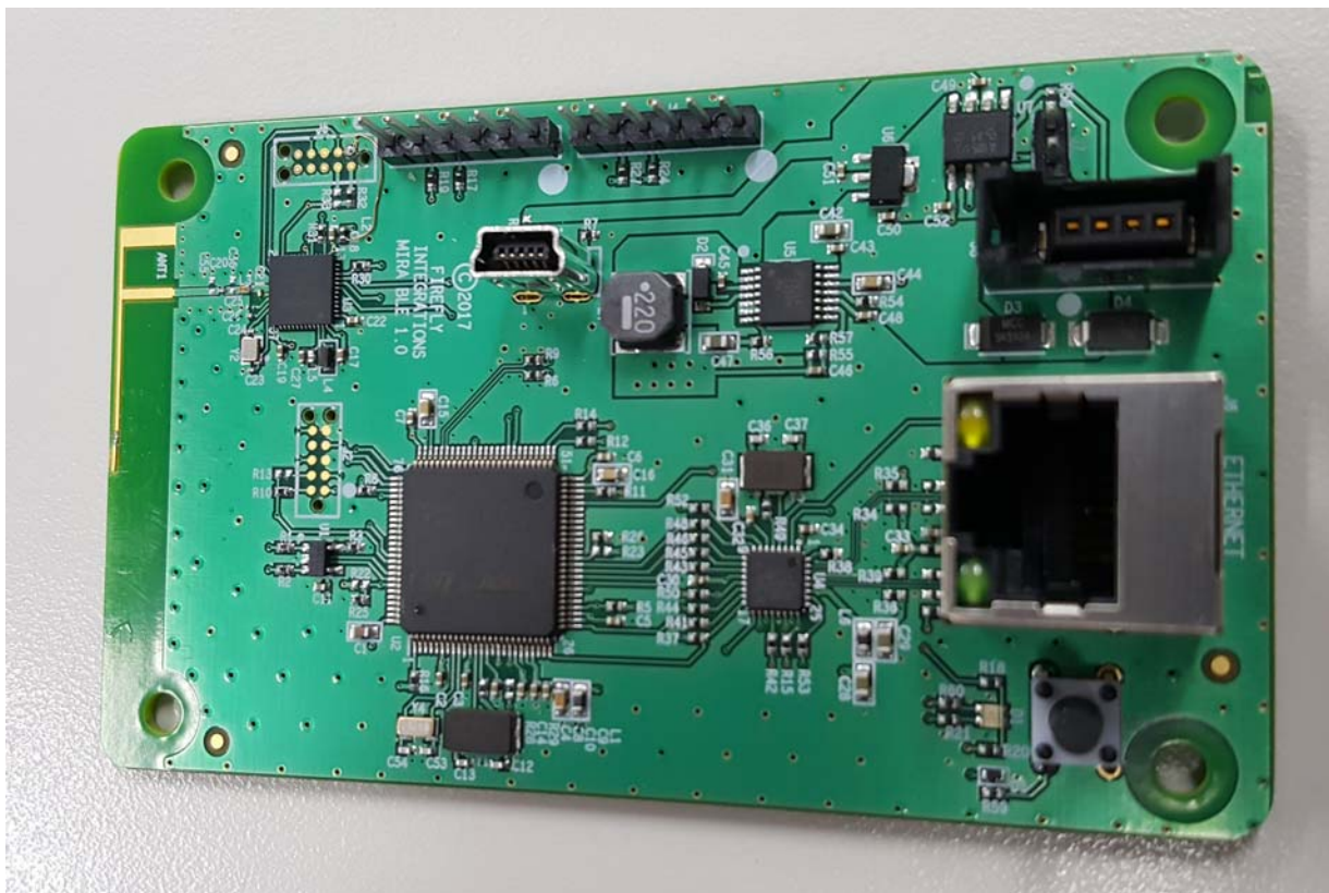
Same PCB; Top view, showing ethernet side
