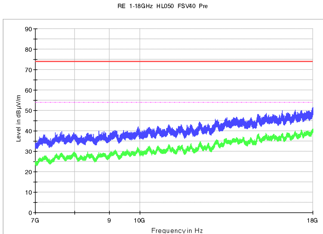
Figure 34: Radiated Spurious Emission, TM2, 7GHz to 18GHz, H
