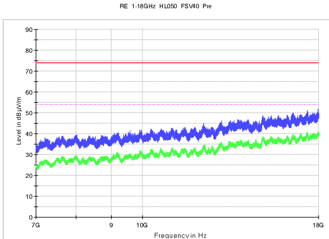
Figure 27: Radiated Spurious Emission, TM1, 7GHz to 18GHz, V
