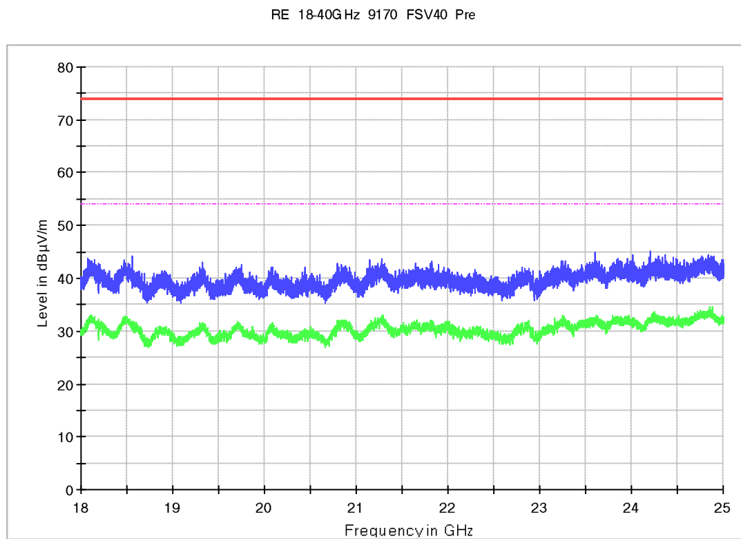
Figure 28: Radiated Spurious Emission, TM1, 18GHz to 25GHz, H
