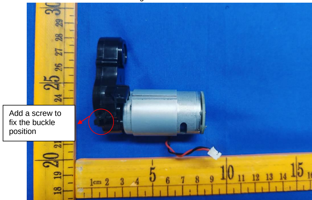
Figure 11. Alternative construction of main brush motor
