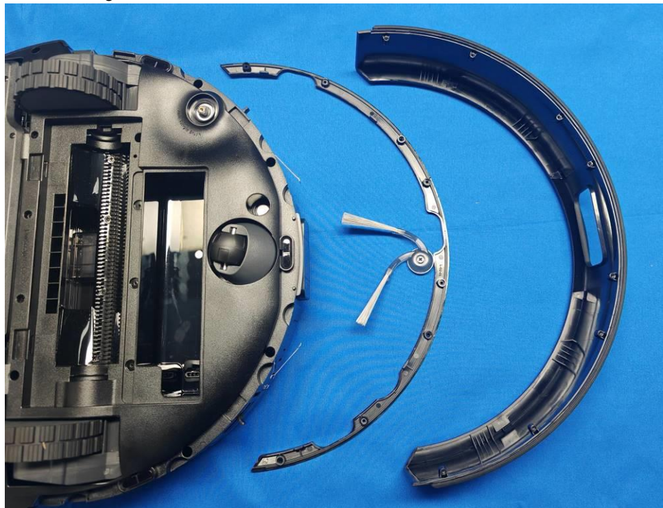
Figure 3. Internal view
