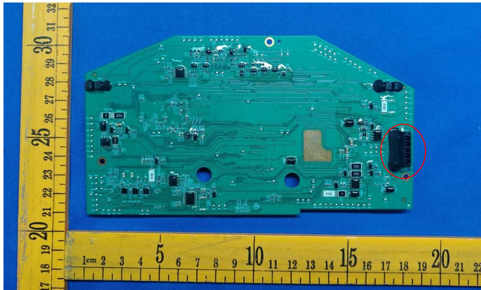
Figure 10. Main PCB
