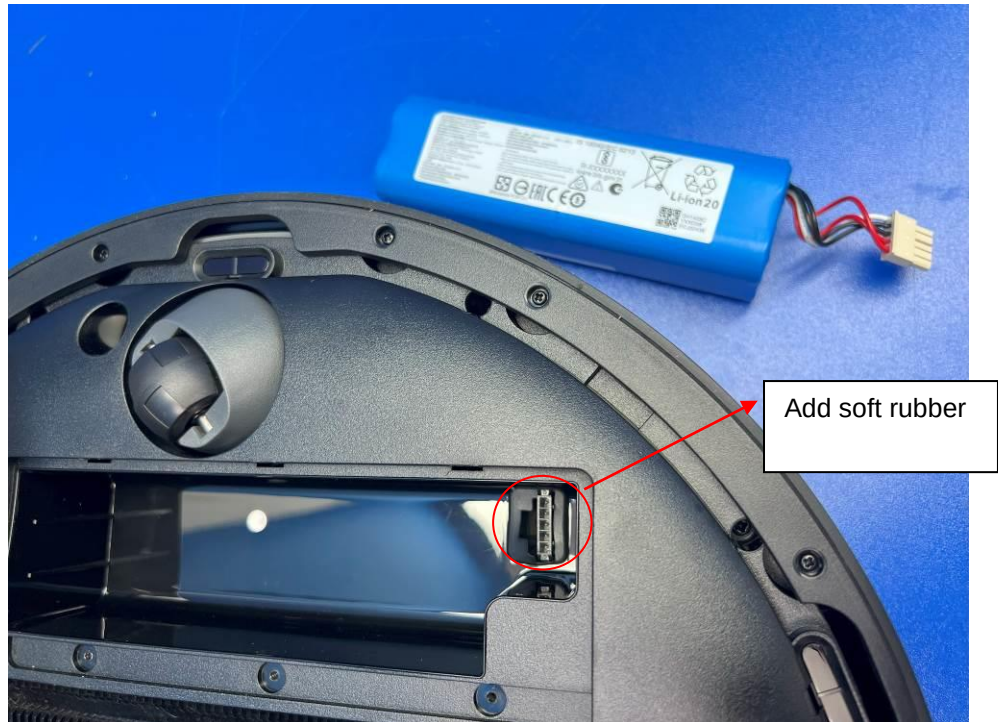
Figure 2. Alternative construction of Robotic Vacuum Cleaner
