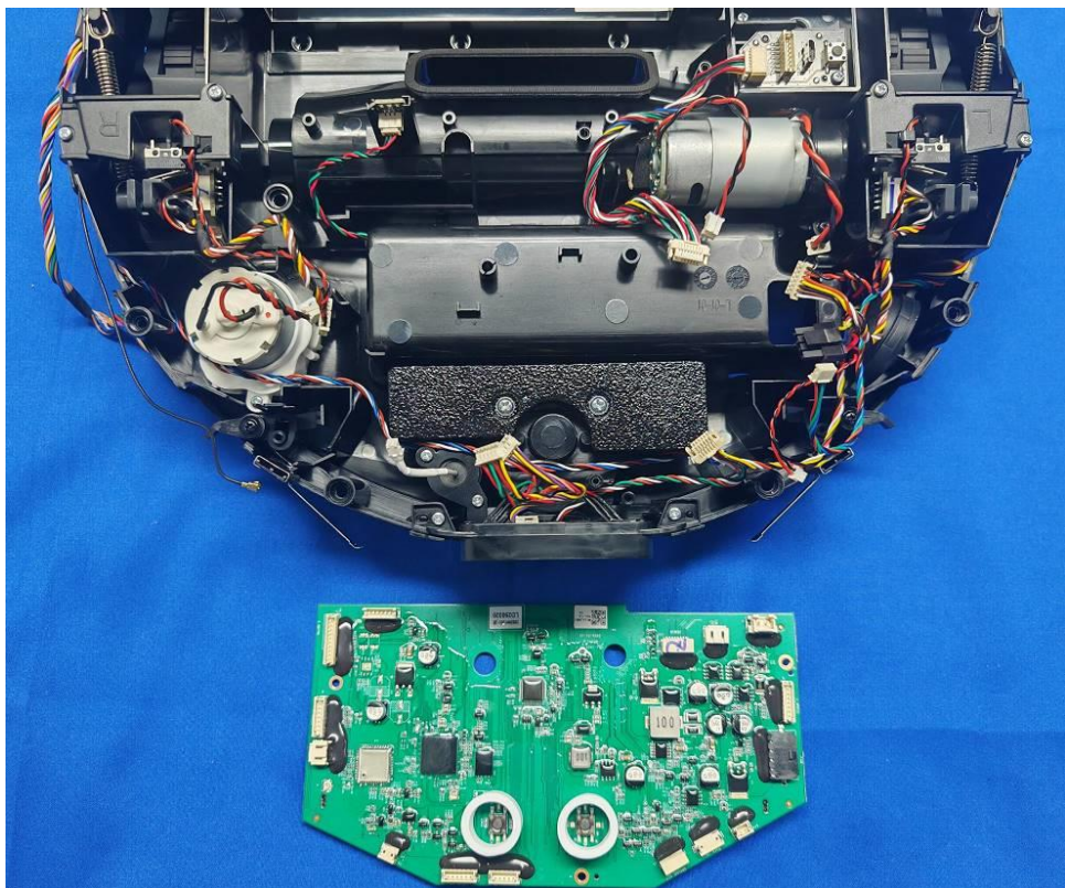
Figure 7. Internal view
