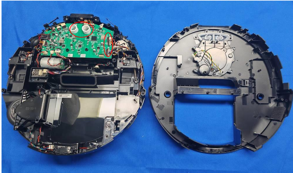
Figure 6. Internal view
