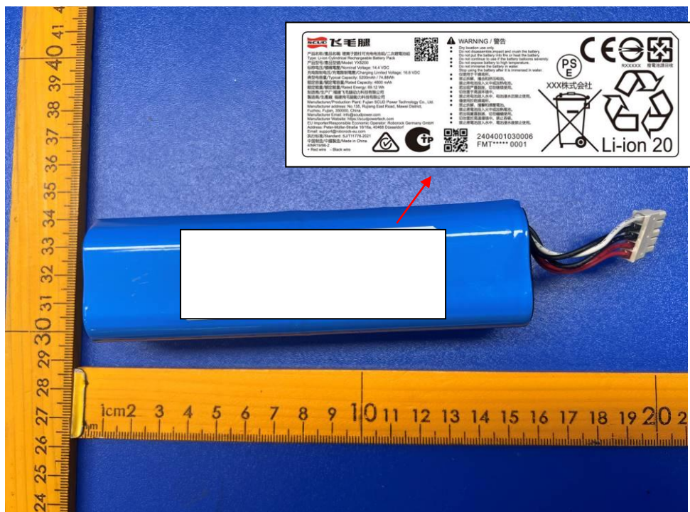
Figure 18. Original Battery pack of model: YX5200 of Robotic Vacuum Cleaner
