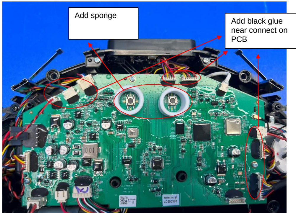
Figure 8. Alternative construction of Robotic Vacuum Cleaner
