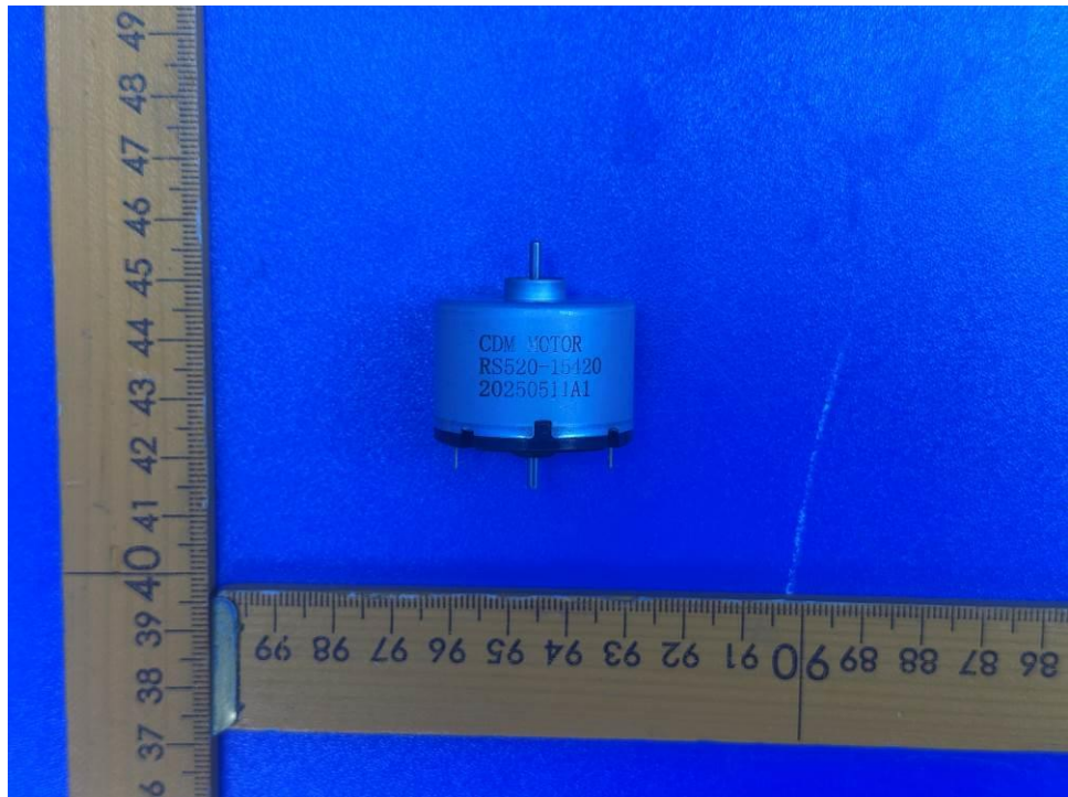
Figure 16. Alternative Wheel motor: RS520-15420 of Robotic Vacuum Cleaner
