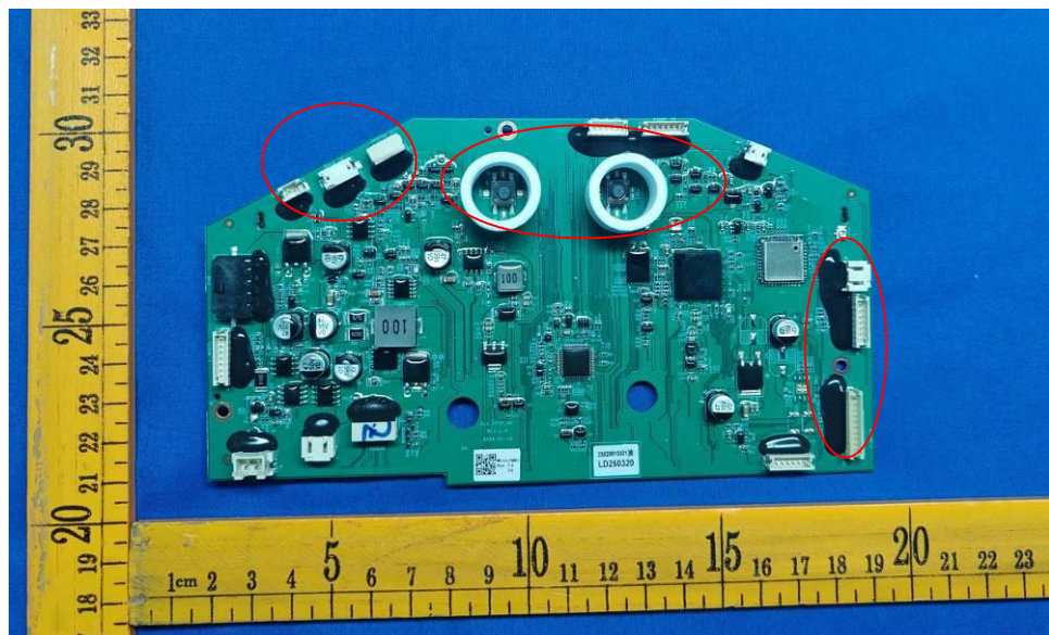
Figure 9. Main PCB
