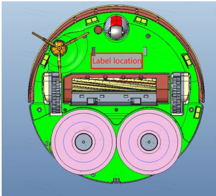
Label location (on the robot cleaner bottom)
