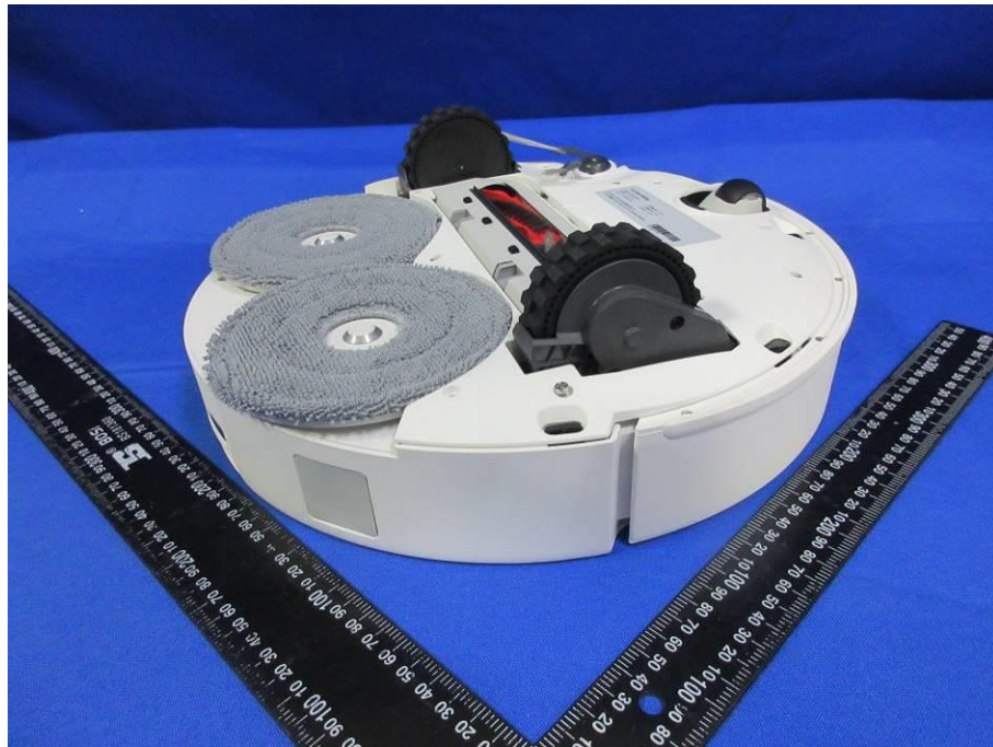
All View of EUT-2
