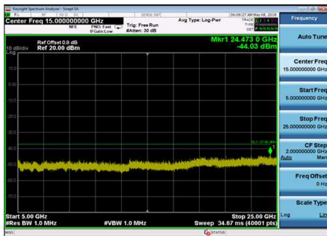
802.11n(HT40),2452MHz,Ant0,Plot 5,5,5000MHz~25000MHz
