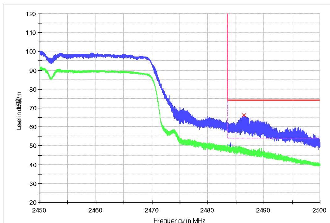
Figure 16: Radiated Band-Edge, n-HT40-2452MHz, V
