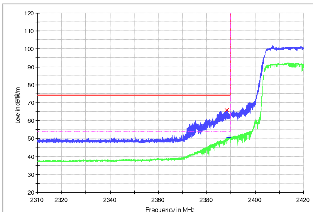
Figure 14: Radiated Band-Edge, n-HT40-2422MHz, V
