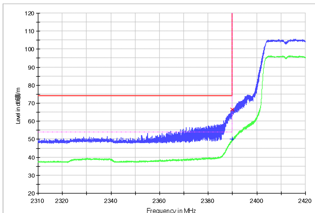
Figure 10: Radiated Band-Edge, n-HT20-2412MHz, V
