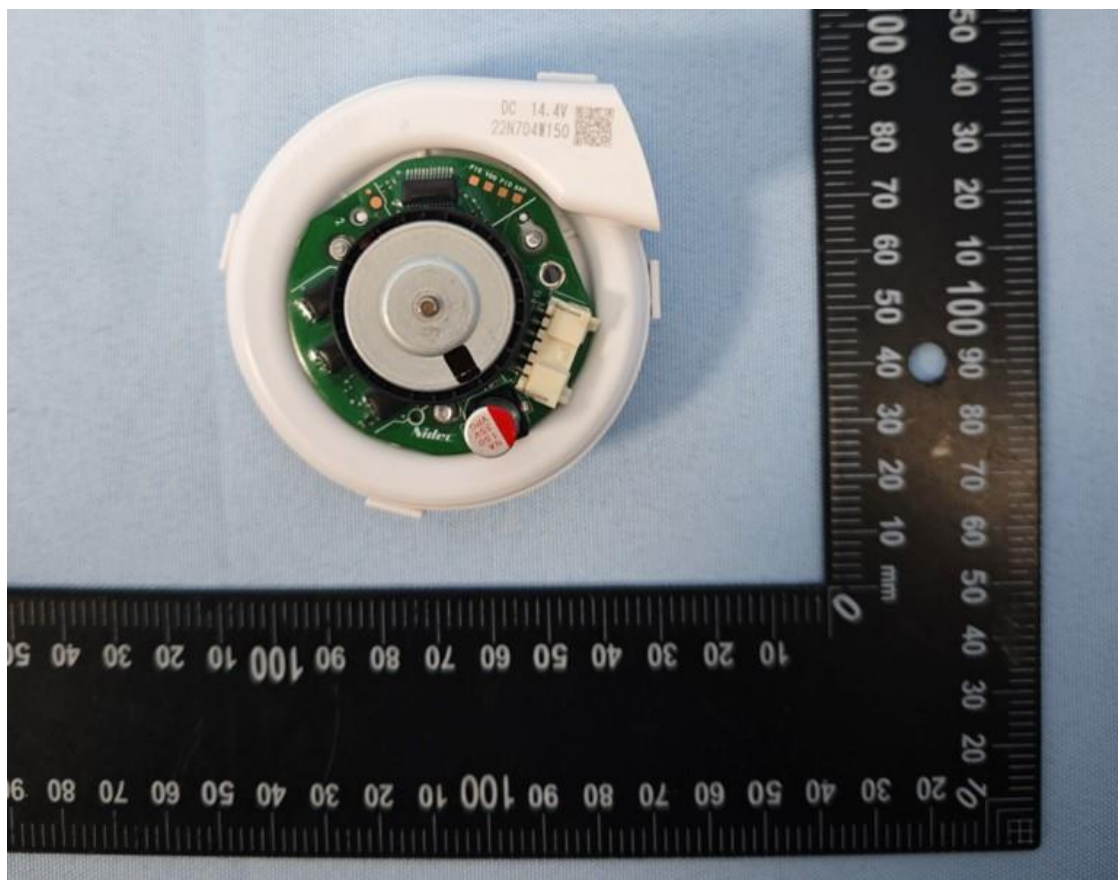
Alternative suction motor 22N704W150
