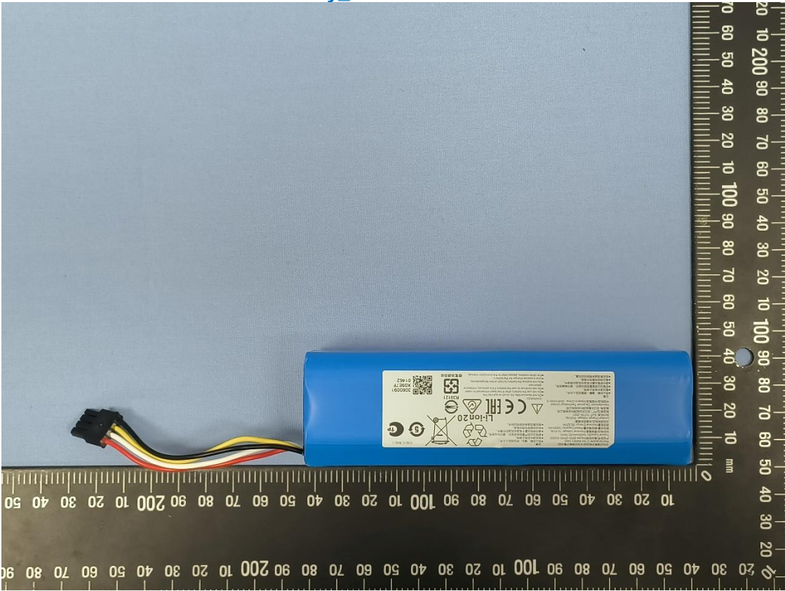
<Battery_BRR-2P4S-6400S>
