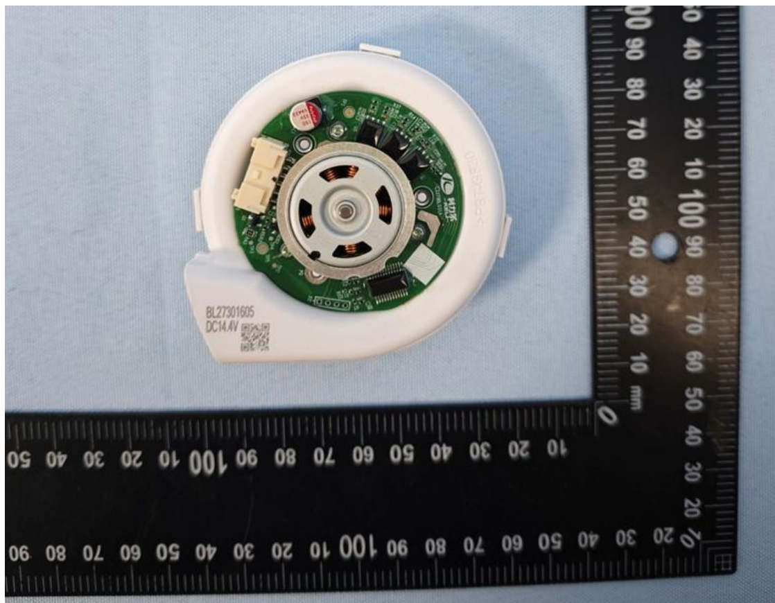
Alternative suction motor BL27301605
