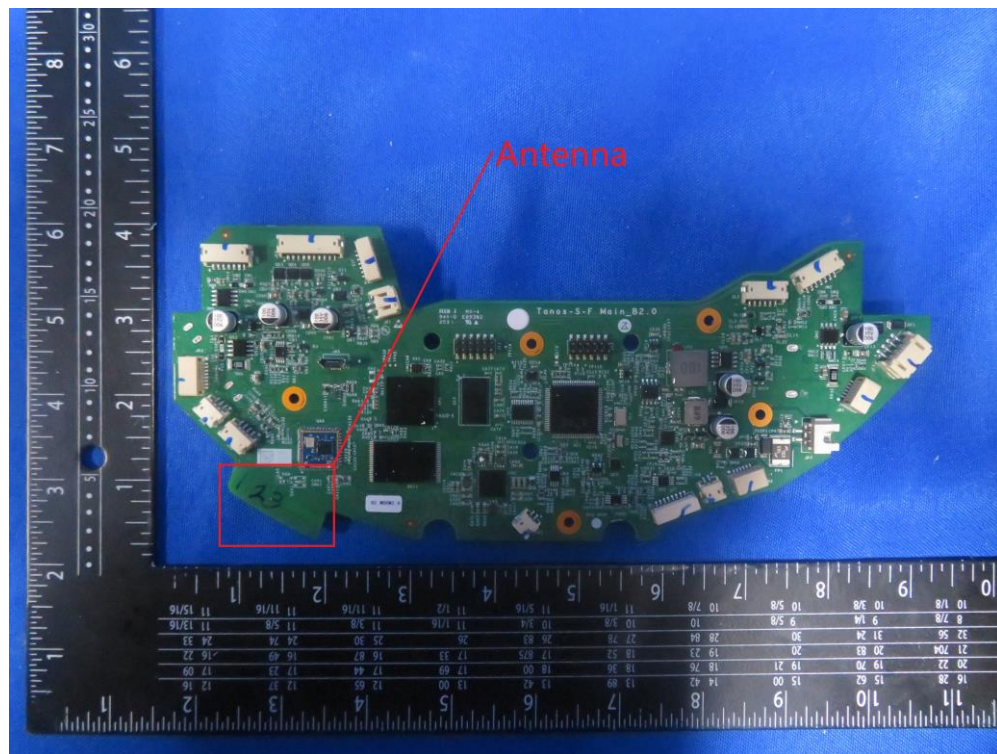
(29) EUT Photo
