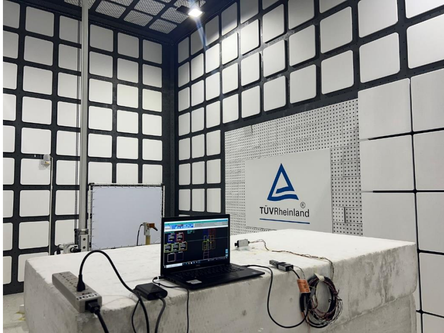
Photograph 7: Test Setup for Spurious Emissions (Back View 5)
