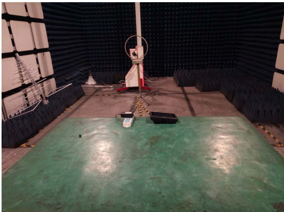
Spurious Emission
