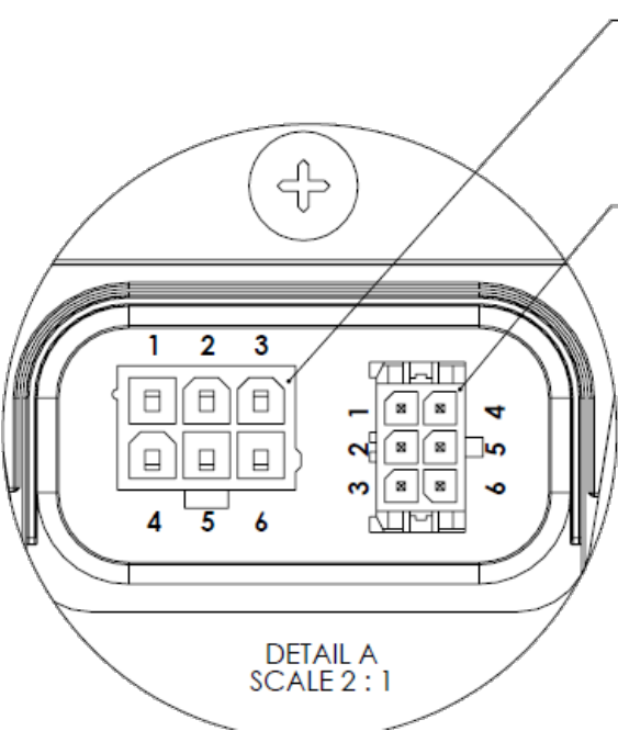
POWER AND MC CONNECTOR
