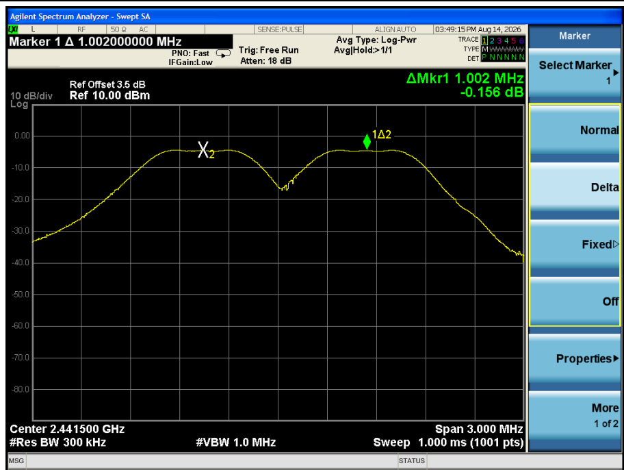
GFSK mode-CH39
