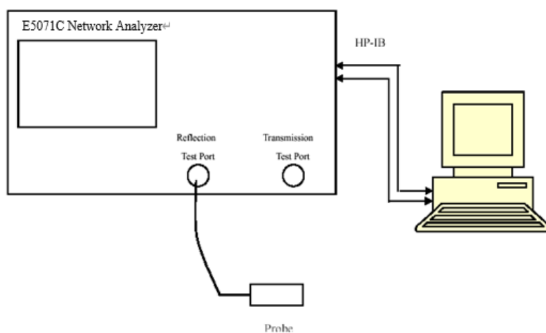
Liquid Verification Setup Block Diagram
