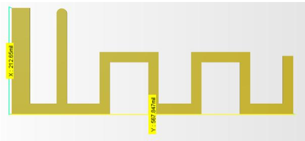
2.4G: 14.42*5.04mm
