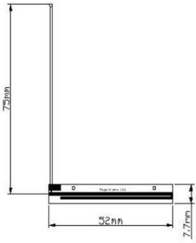
LoRa: 52*7.7mm
