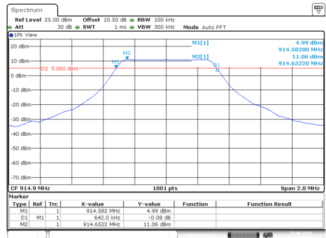
500K_High_Channel
