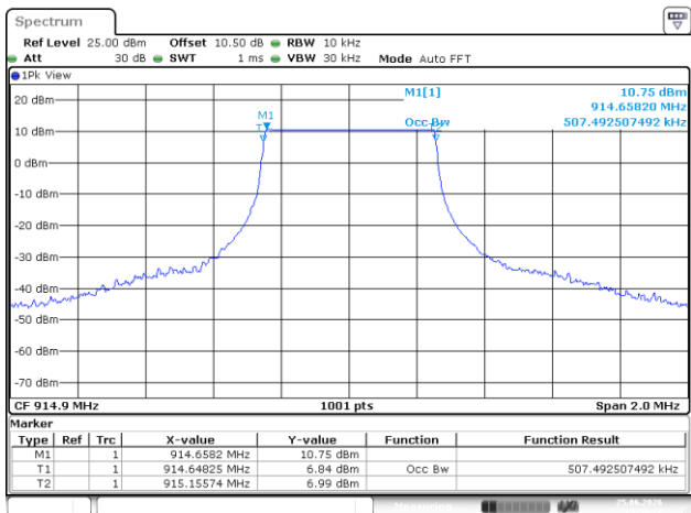
500K_High_Channel
