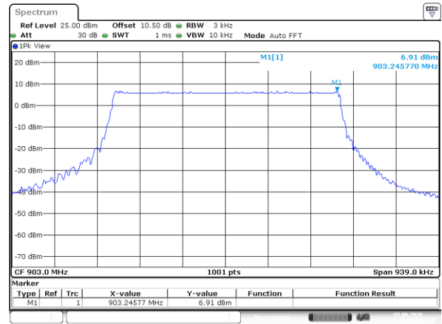
500K_Low_Channel
