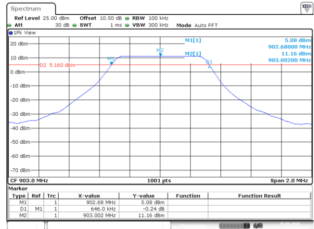
500K_Low_Channel
