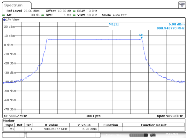
500K_Middle_Channel
