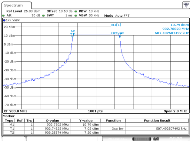
500K_Low_Channel
