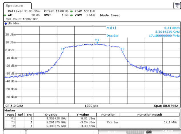
802.11a_5300MHz
