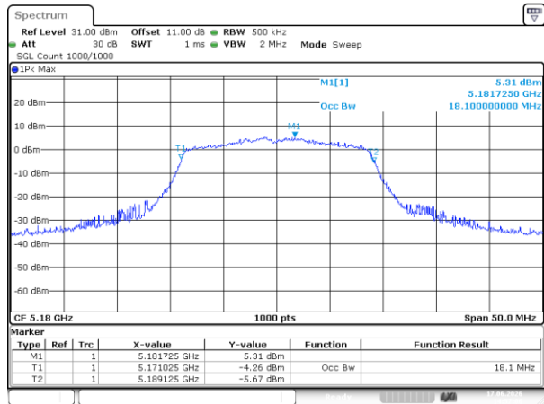
802.11n20_5180MHz
