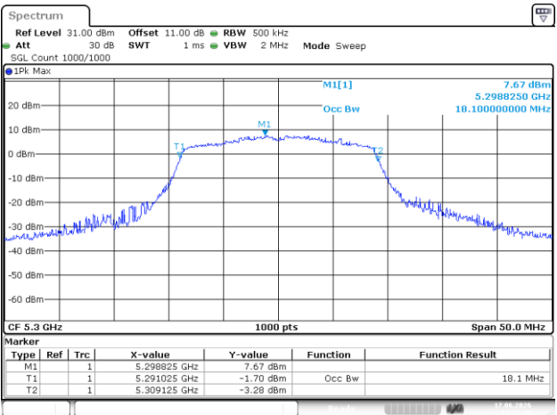
802.11n20_5300MHz
