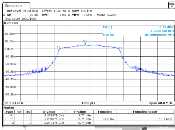
802.11n20_5240MHz
