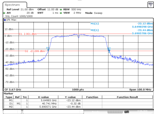
802.11n40_5670MHz
