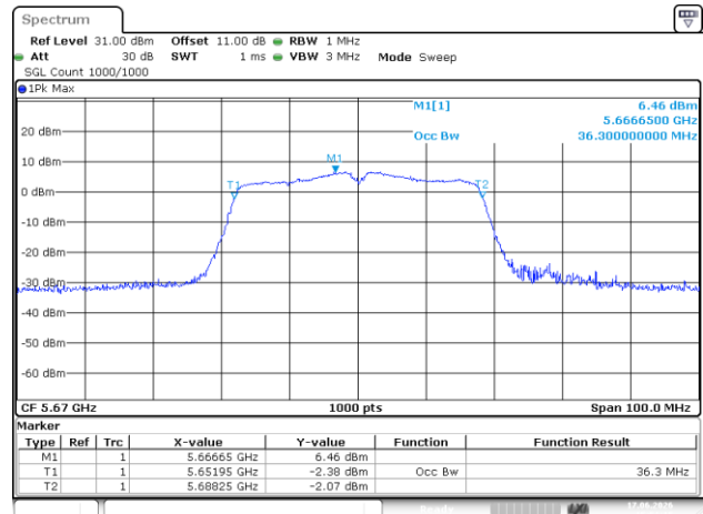
802.11n40_5670MHz
