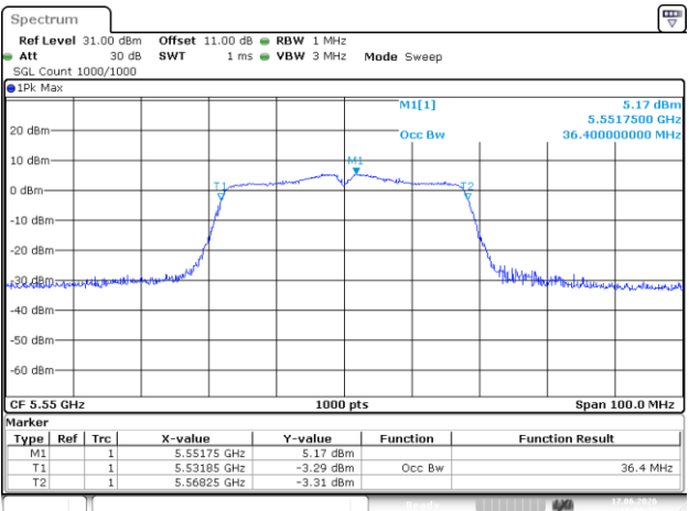
802.11n40_5550MHz
